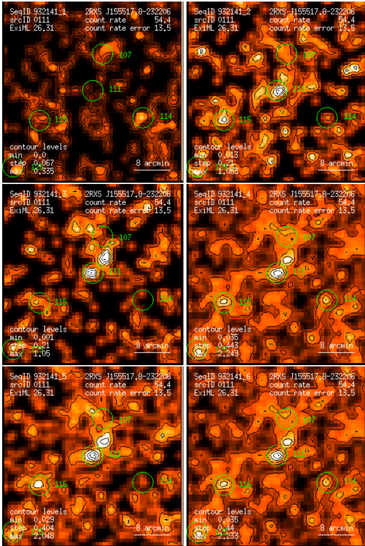
Figure 111: RASS 932141: detection 0111: band rate images, Gaussian filter: (1) PSPC channels 11 – 41, (2) 52 – 90, (3) 91 – 201, (4) 11 – 235, (5) 52 – 201, (6) 11 – 201. Broad band rates in counts/ks. Band rate contour levels in counts/ks/arcmin 2 .
