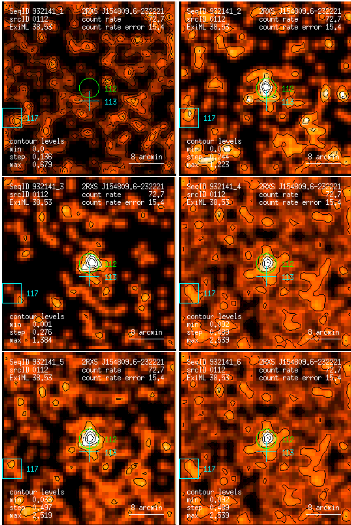
Figure 112: RASS 932141: detection 0112: band rate images, Gaussian filter: (1) PSPC channels 11 – 41, (2) 52 – 90, (3) 91 – 201, (4) 11 – 235, (5) 52 – 201, (6) 11 – 201. Broad band rates in counts/ks. Band rate contour levels in counts/ks/arcmin 2 .
