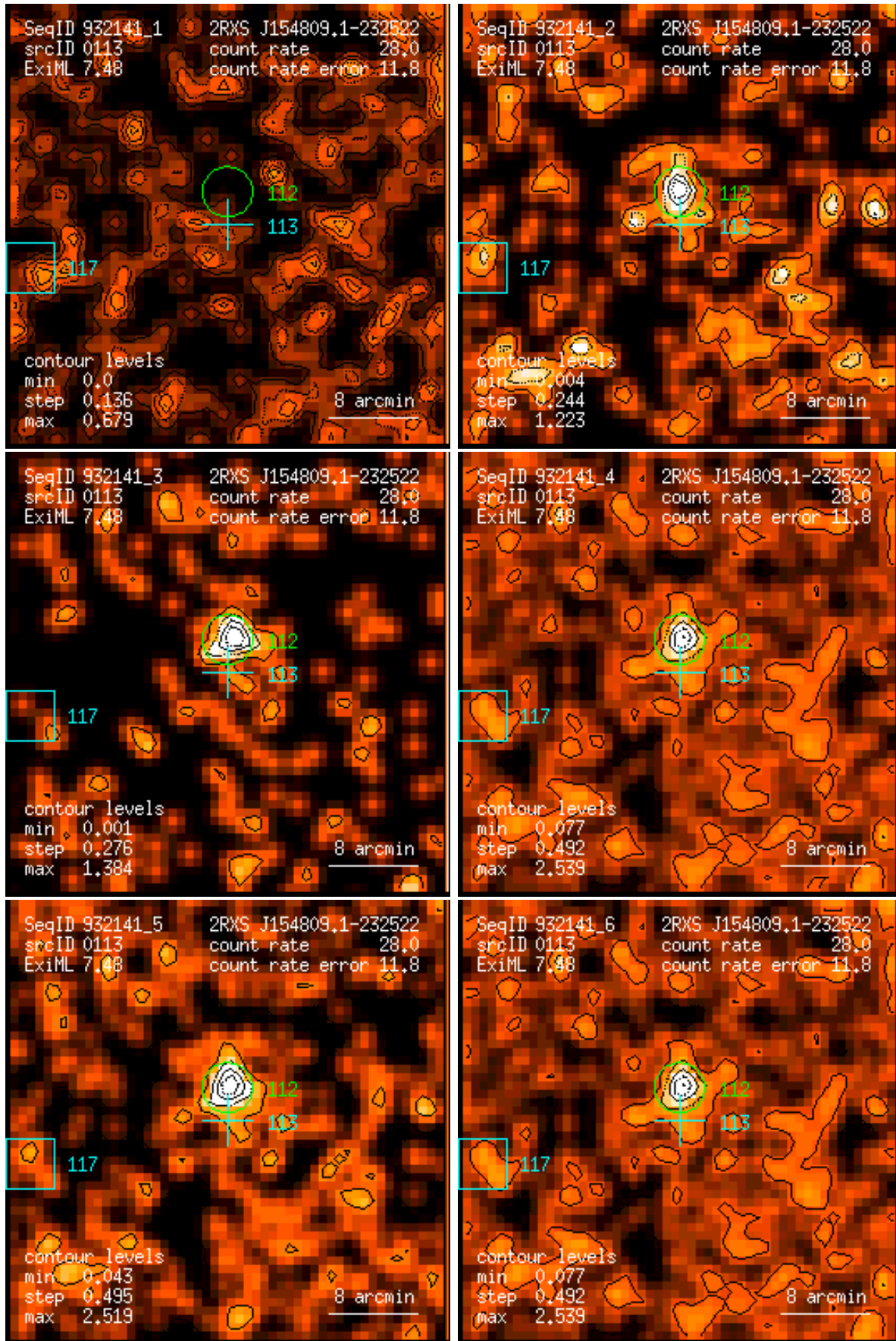
Figure 113: RASS 932141: detection 0113: band rate images, Gaussian filter: (1) PSPC channels 11 – 41, (2) 52 – 90, (3) 91 – 201, (4) 11 – 235, (5) 52 – 201, (6) 11 – 201. Broad band rates in counts/ks. Band rate contour levels in counts/ks/arcmin 2 .
