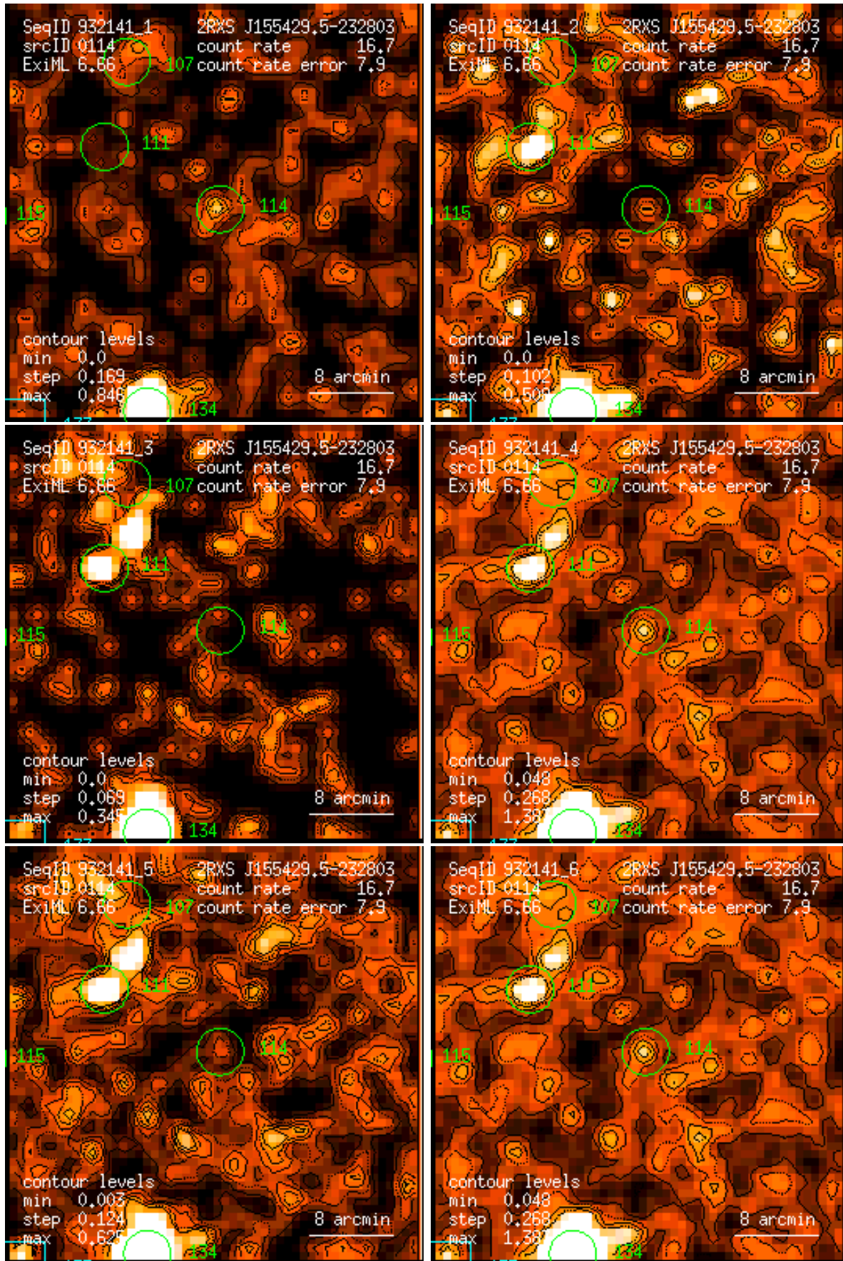
Figure 114: RASS 932141: detection 0114: band rate images, Gaussian filter: (1) PSPC channels 11 – 41, (2) 52 – 90, (3) 91 – 201, (4) 11 – 235, (5) 52 – 201, (6) 11 – 201. Broad band rates in counts/ks. Band rate contour levels in counts/ks/arcmin 2 .
