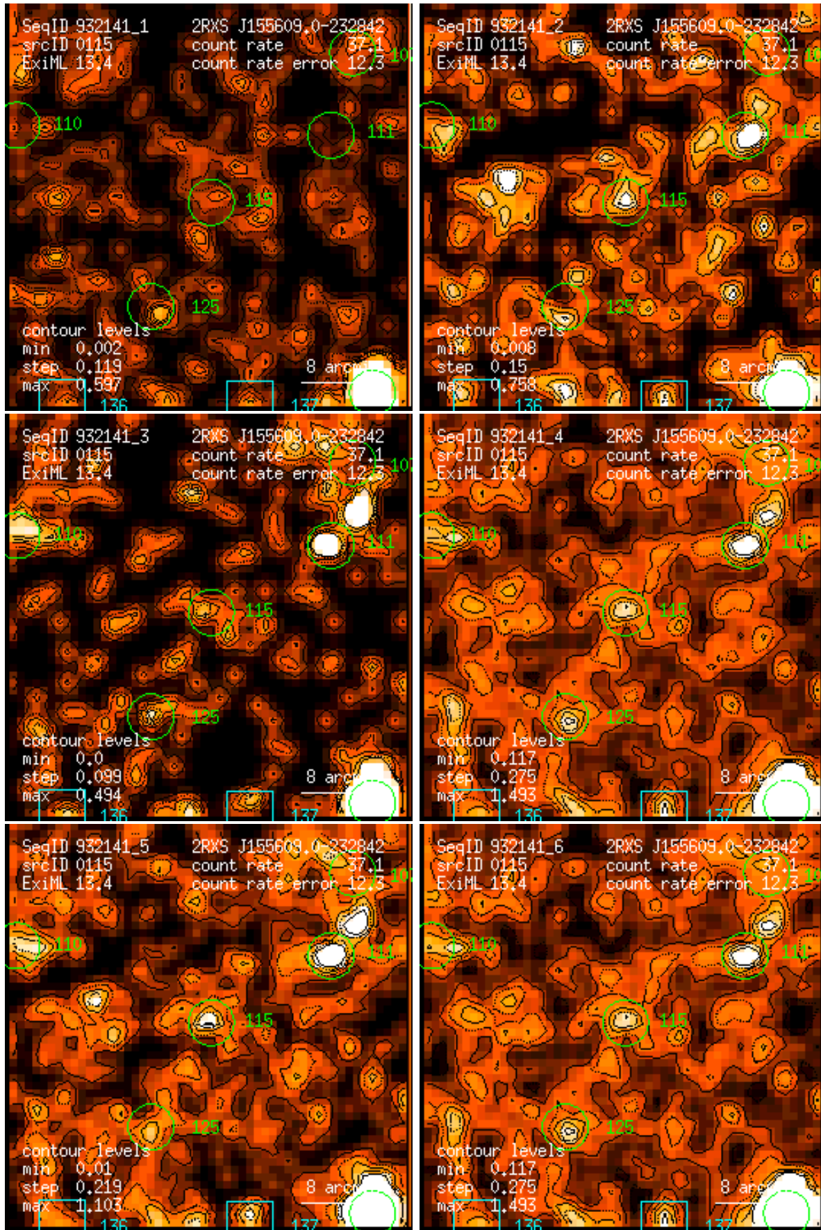
Figure 115: RASS 932141: detection 0115: band rate images, Gaussian filter: (1) PSPC channels 11 – 41, (2) 52 – 90, (3) 91 – 201, (4) 11 – 235, (5) 52 – 201, (6) 11 – 201. Broad band rates in counts/ks. Band rate contour levels in counts/ks/arcmin 2 .
