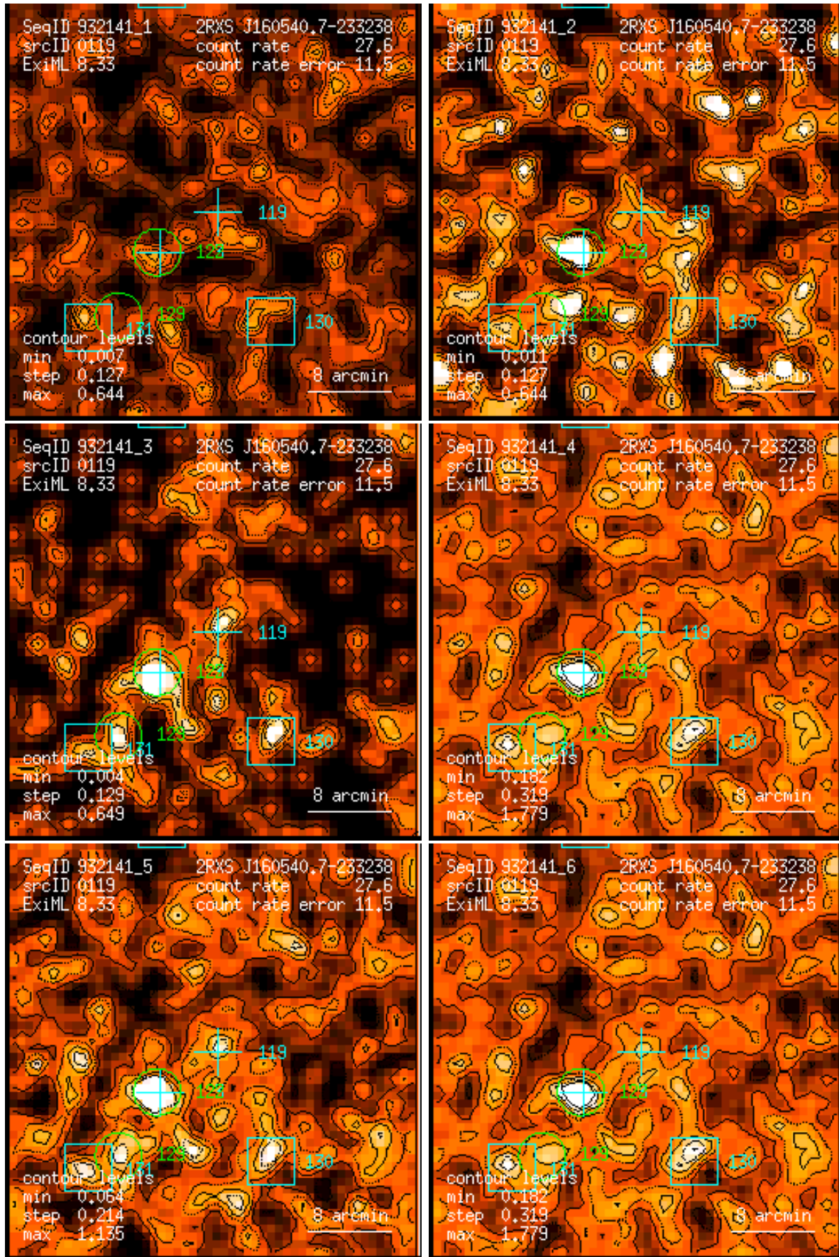
Figure 119: RASS 932141: detection 0119: band rate images, Gaussian filter: (1) PSPC channels 11 – 41, (2) 52 – 90, (3) 91 – 201, (4) 11 – 235, (5) 52 – 201, (6) 11 – 201. Broad band rates in counts/ks. Band rate contour levels in counts/ks/arcmin 2 .
