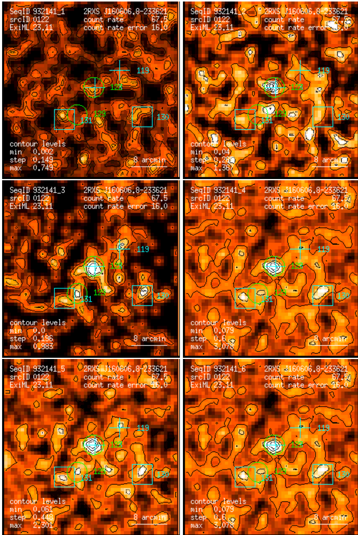
Figure 122: RASS 932141: detection 0122: band rate images, Gaussian filter: (1) PSPC channels 11 – 41, (2) 52 – 90, (3) 91 – 201, (4) 11 – 235, (5) 52 – 201, (6) 11 – 201. Broad band rates in counts/ks. Band rate contour levels in counts/ks/arcmin 2 .
