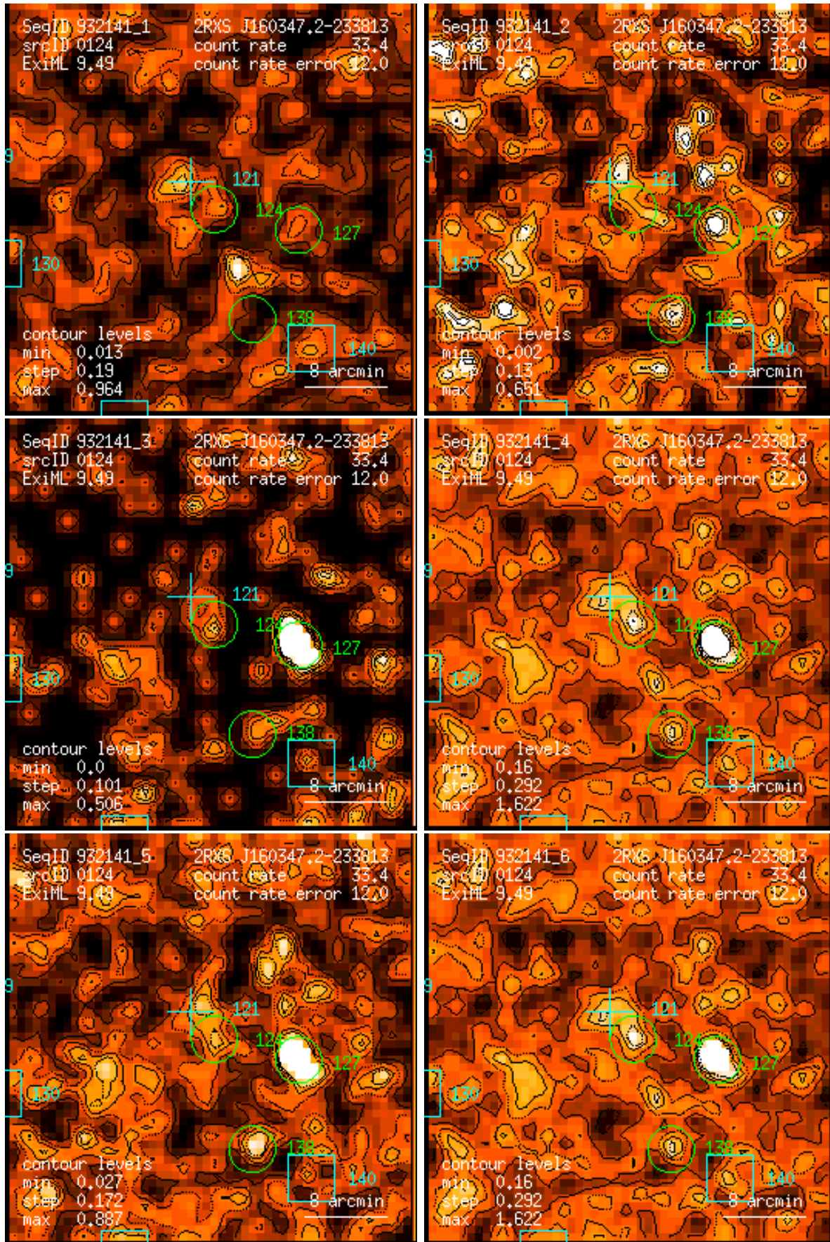
Figure 124: RASS 932141: detection 0124: band rate images, Gaussian filter: (1) PSPC channels 11 – 41, (2) 52 – 90, (3) 91 – 201, (4) 11 – 235, (5) 52 – 201, (6) 11 – 201. Broad band rates in counts/ks. Band rate contour levels in counts/ks/arcmin 2 .
