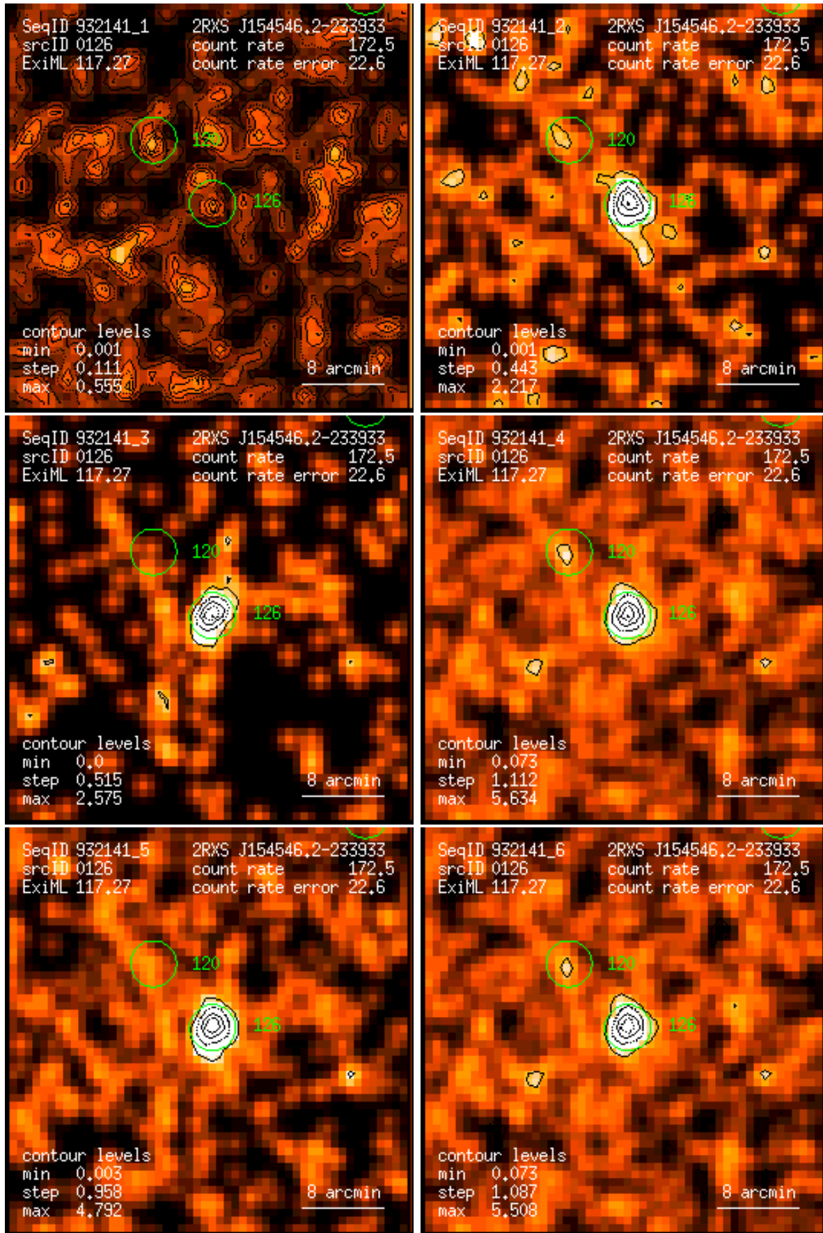
Figure 126: RASS 932141: detection 0126: band rate images, Gaussian filter: (1) PSPC channels 11 – 41, (2) 52 – 90, (3) 91 – 201, (4) 11 – 235, (5) 52 – 201, (6) 11 – 201. Broad band rates in counts/ks. Band rate contour levels in counts/ks/arcmin 2 .
