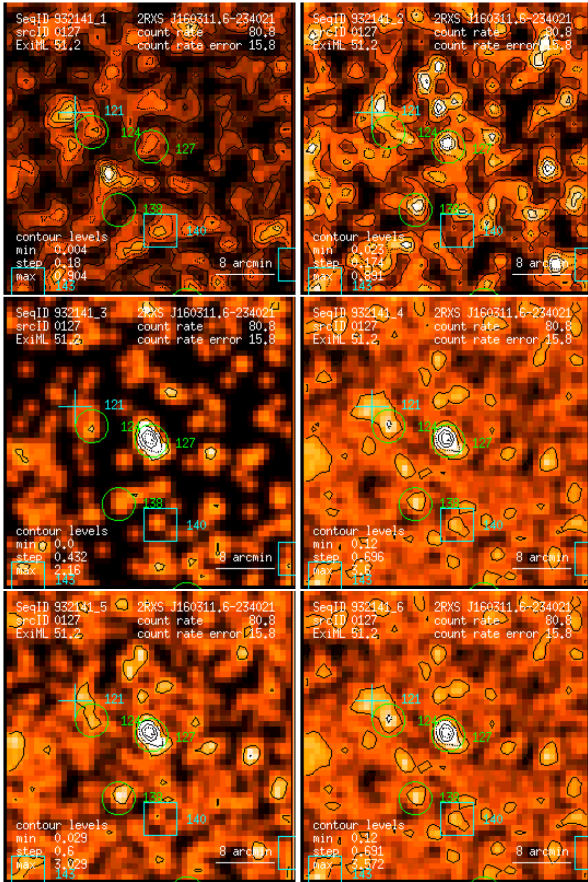
Figure 127: RASS 932141: detection 0127: band rate images, Gaussian filter: (1) PSPC channels 11 – 41, (2) 52 – 90, (3) 91 – 201, (4) 11 – 235, (5) 52 – 201, (6) 11 – 201. Broad band rates in counts/ks. Band rate contour levels in counts/ks/arcmin 2 .
