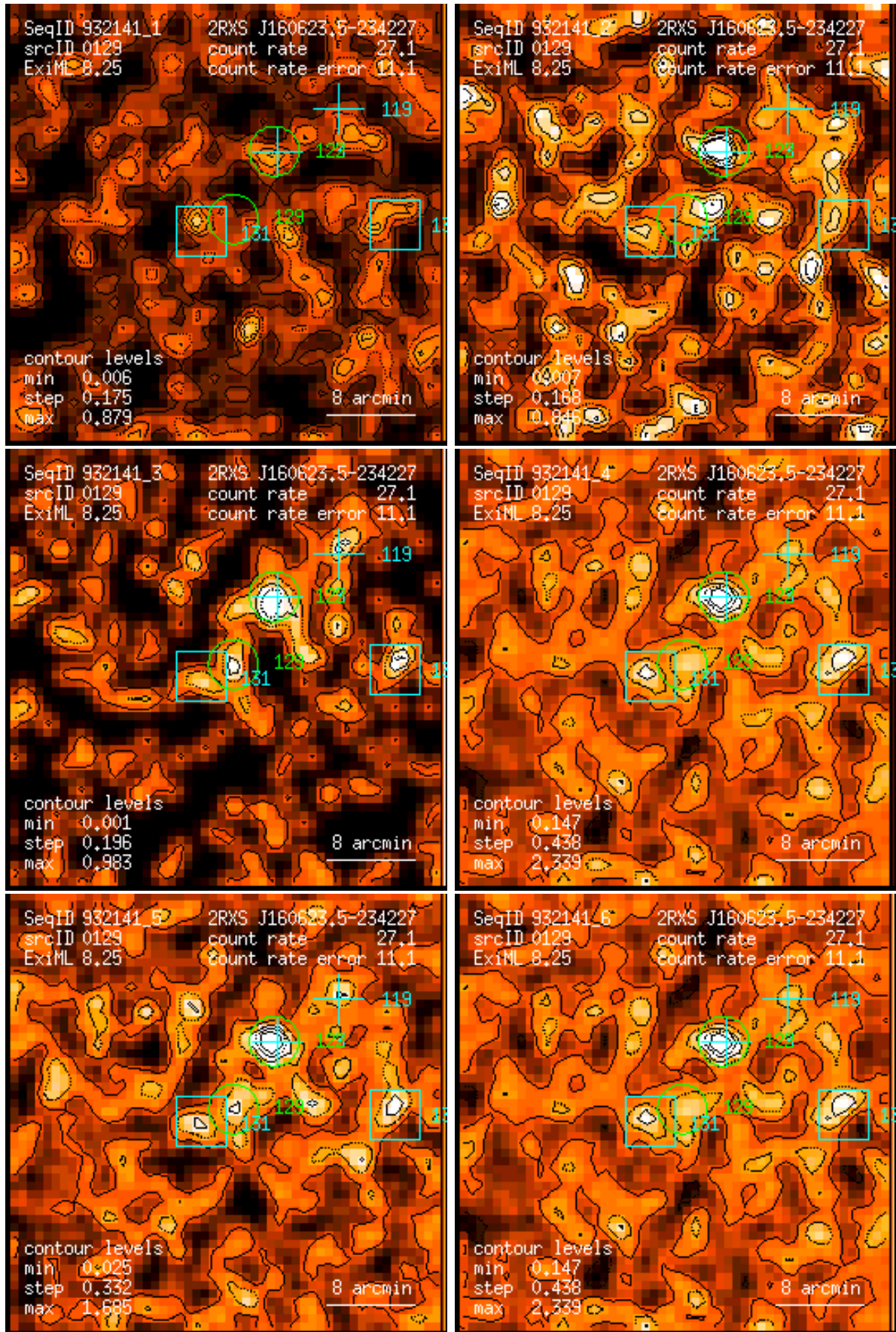
Figure 129: RASS 932141: detection 0129: band rate images, Gaussian filter: (1) PSPC channels 11 – 41, (2) 52 – 90, (3) 91 – 201, (4) 11 – 235, (5) 52 – 201, (6) 11 – 201. Broad band rates in counts/ks. Band rate contour levels in counts/ks/arcmin 2 .
