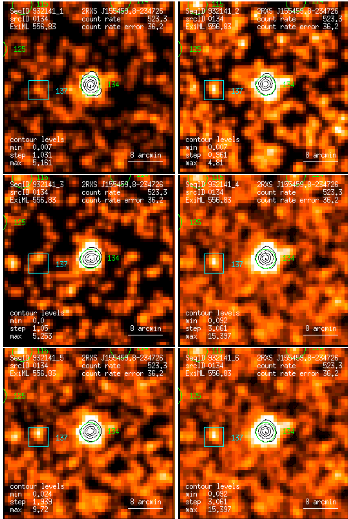
Figure 134: RASS 932141: detection 0134: band rate images, Gaussian filter: (1) PSPC channels 11 – 41, (2) 52 – 90, (3) 91 – 201, (4) 11 – 235, (5) 52 – 201, (6) 11 – 201. Broad band rates in counts/ks. Band rate contour levels in counts/ks/arcmin 2 .
