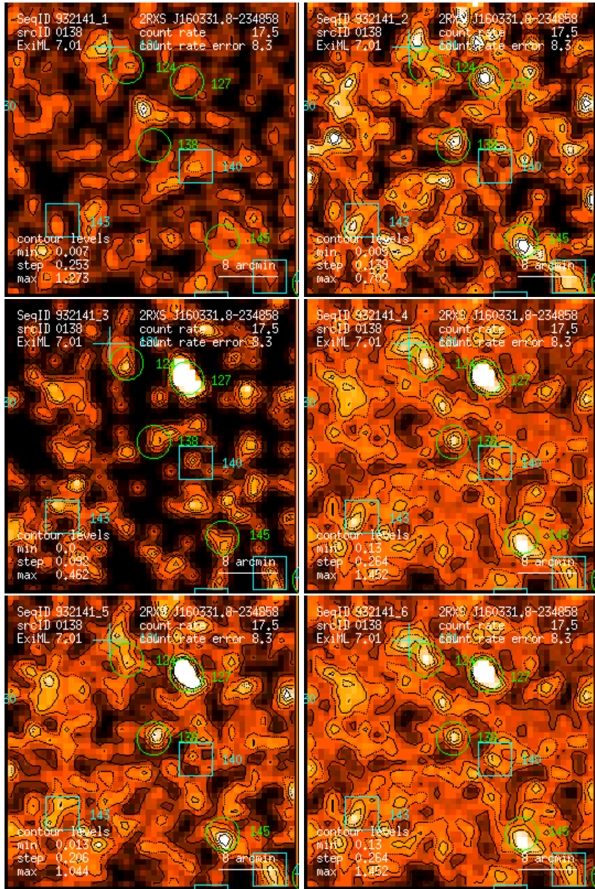
Figure 138: RASS 932141: detection 0138: band rate images, Gaussian filter: (1) PSPC channels 11 – 41, (2) 52 – 90, (3) 91 – 201, (4) 11 – 235, (5) 52 – 201, (6) 11 – 201. Broad band rates in counts/ks. Band rate contour levels in counts/ks/arcmin 2 .
