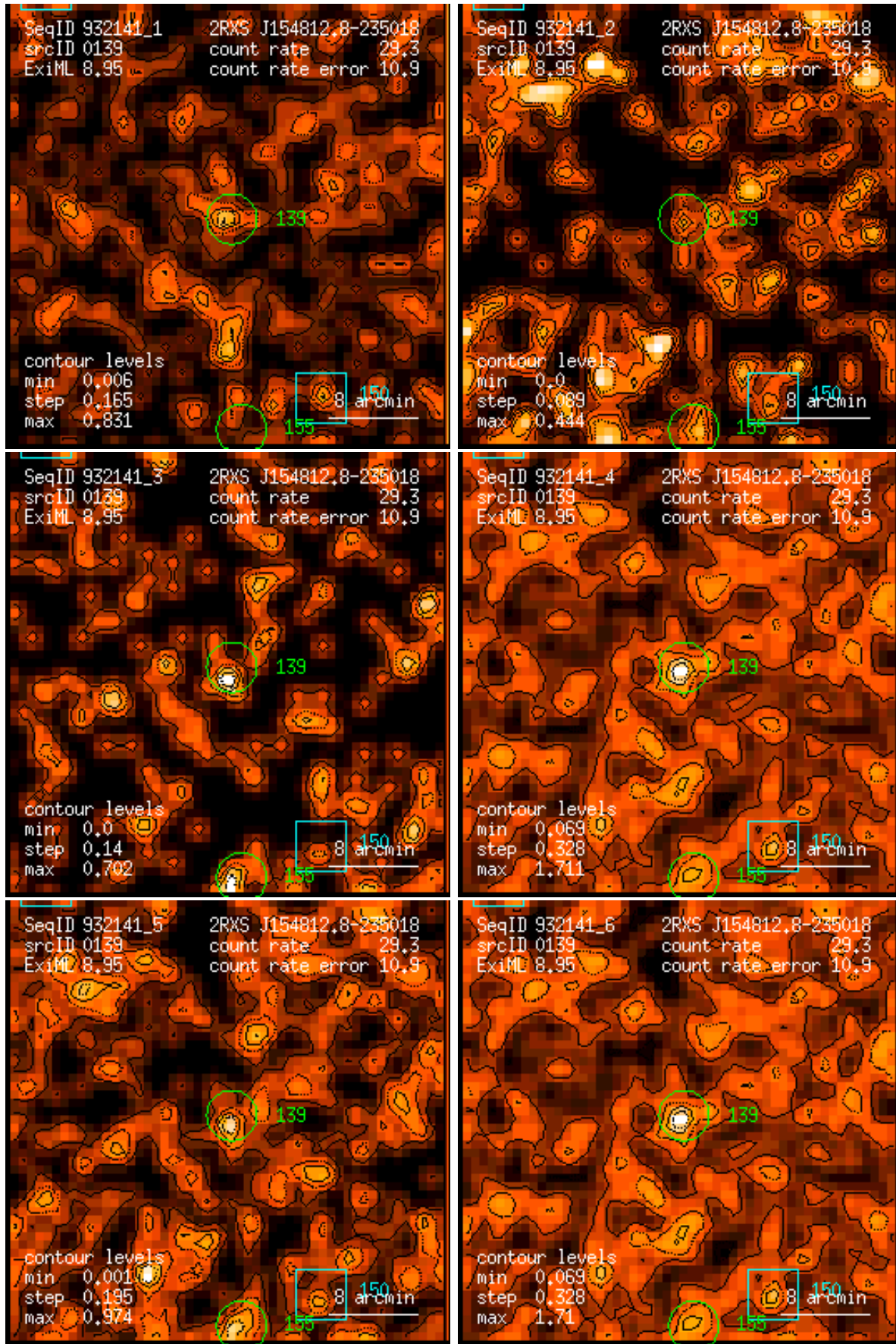
Figure 139: RASS 932141: detection 0139: band rate images, Gaussian filter: (1) PSPC channels 11 – 41, (2) 52 – 90, (3) 91 – 201, (4) 11 – 235, (5) 52 – 201, (6) 11 – 201. Broad band rates in counts/ks. Band rate contour levels in counts/ks/arcmin 2 .
