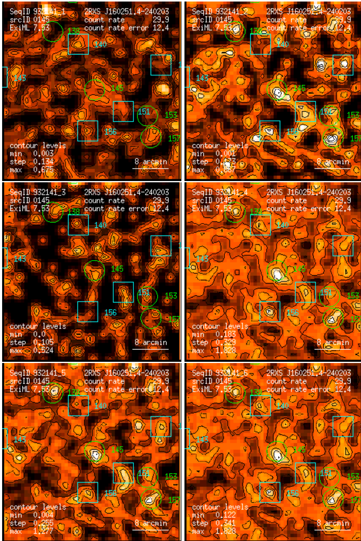
Figure 145: RASS 932141: detection 0145: band rate images, Gaussian filter: (1) PSPC channels 11 – 41, (2) 52 – 90, (3) 91 – 201, (4) 11 – 235, (5) 52 – 201, (6) 11 – 201. Broad band rates in counts/ks. Band rate contour levels in counts/ks/arcmin 2 .
