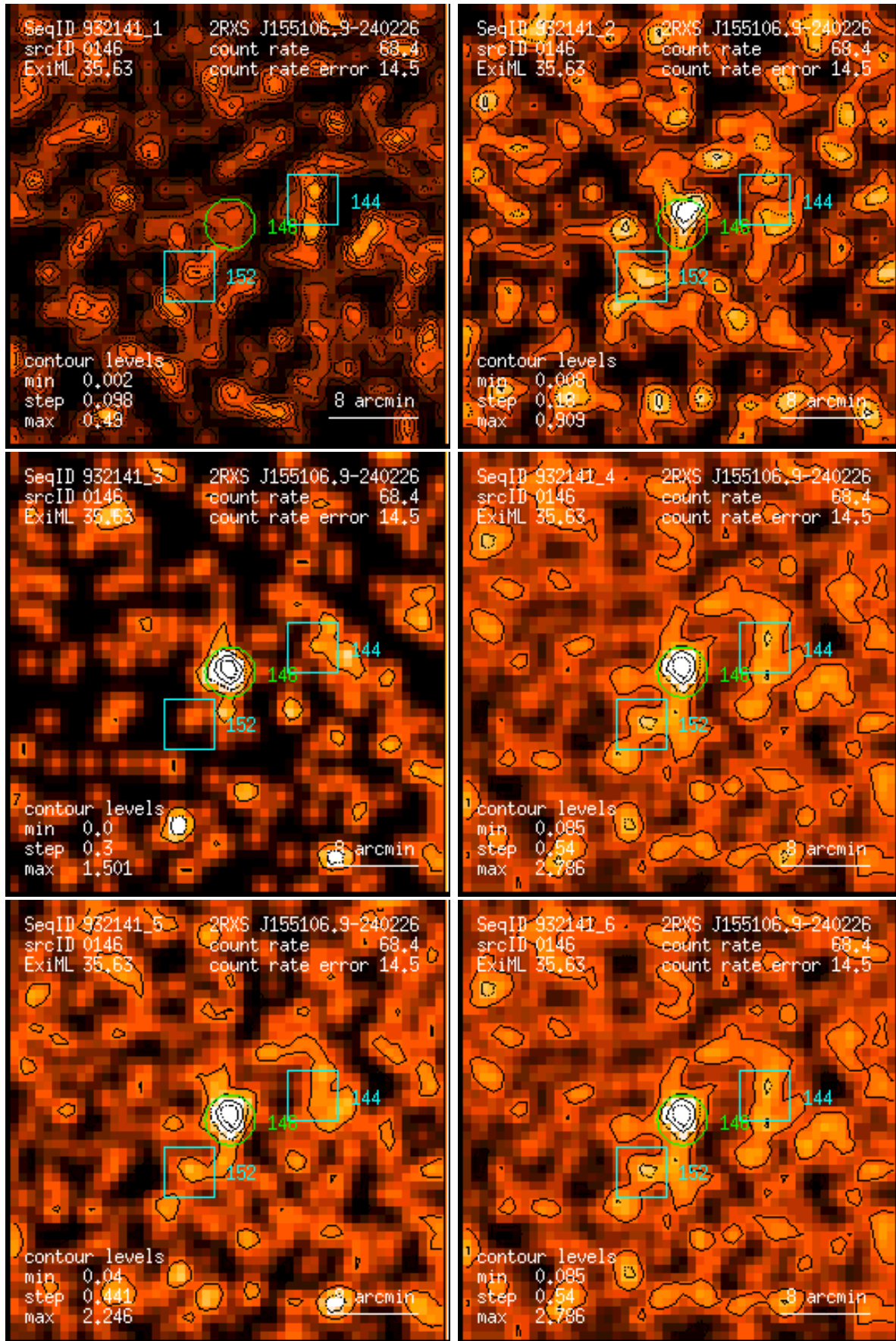
Figure 146: RASS 932141: detection 0146: band rate images, Gaussian filter: (1) PSPC channels 11 – 41, (2) 52 – 90, (3) 91 – 201, (4) 11 – 235, (5) 52 – 201, (6) 11 – 201. Broad band rates in counts/ks. Band rate contour levels in counts/ks/arcmin 2 .
