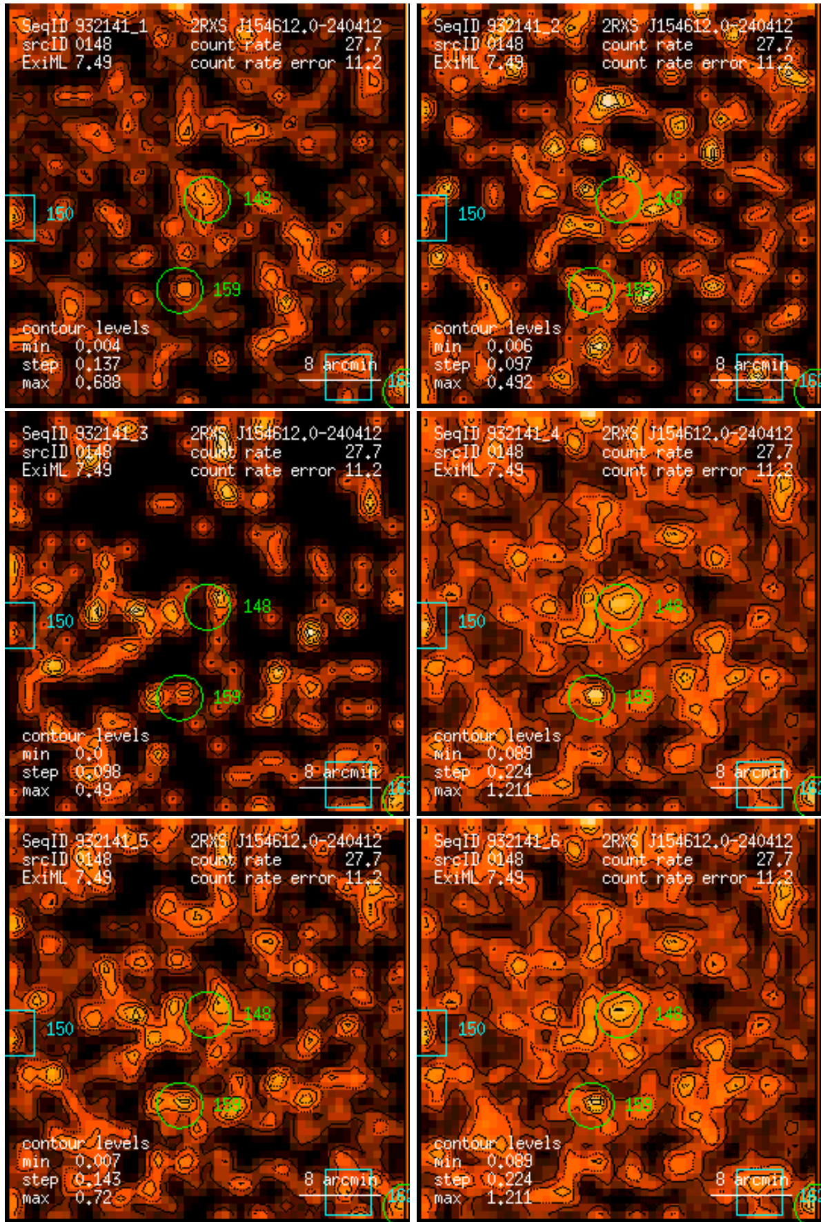
Figure 148: RASS 932141: detection 0148: band rate images, Gaussian filter: (1) PSPC channels 11 – 41, (2) 52 – 90, (3) 91 – 201, (4) 11 – 235, (5) 52 – 201, (6) 11 – 201. Broad band rates in counts/ks. Band rate contour levels in counts/ks/arcmin 2 .
