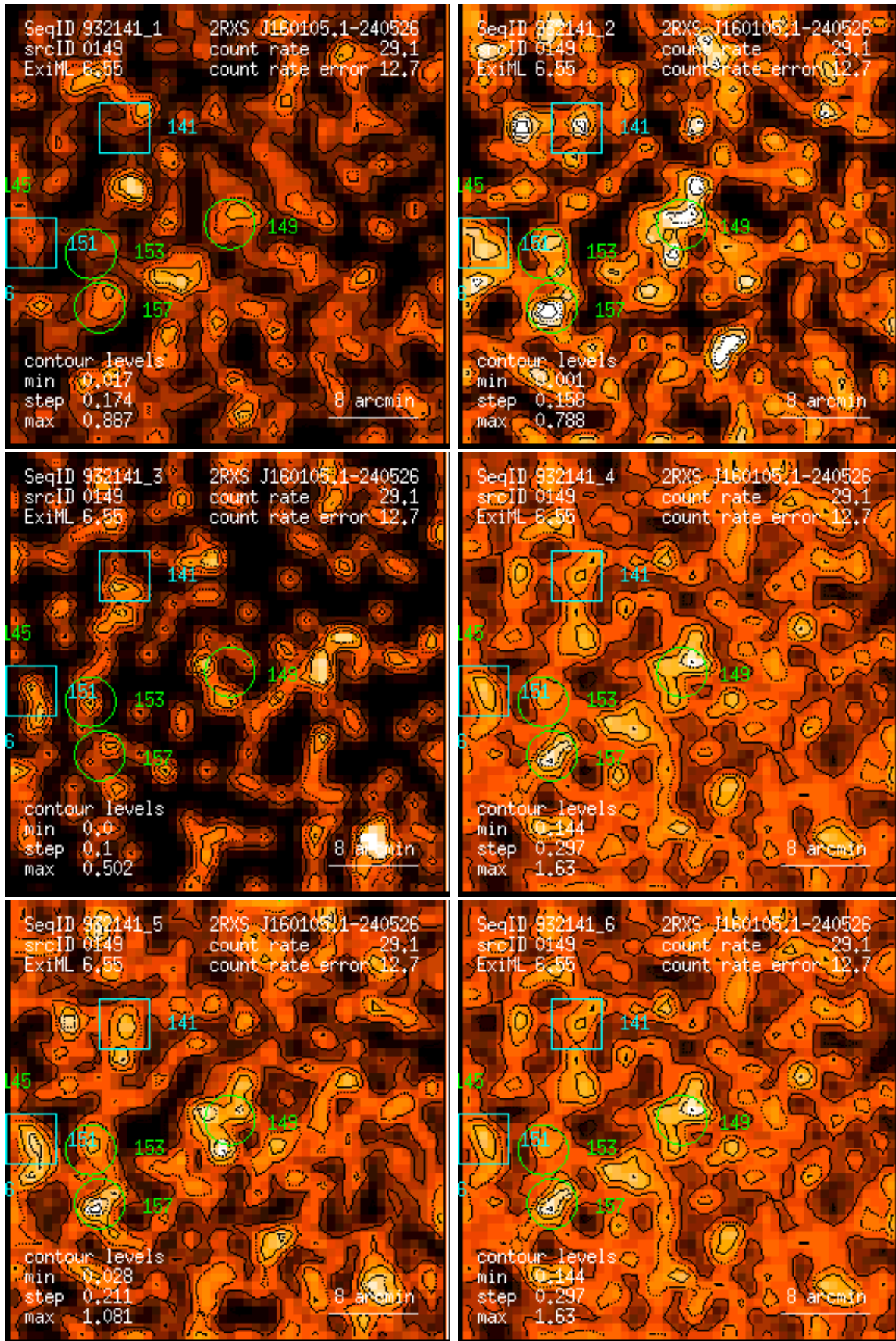
Figure 149: RASS 932141: detection 0149: band rate images, Gaussian filter: (1) PSPC channels 11 – 41, (2) 52 – 90, (3) 91 – 201, (4) 11 – 235, (5) 52 – 201, (6) 11 – 201. Broad band rates in counts/ks. Band rate contour levels in counts/ks/arcmin 2 .
