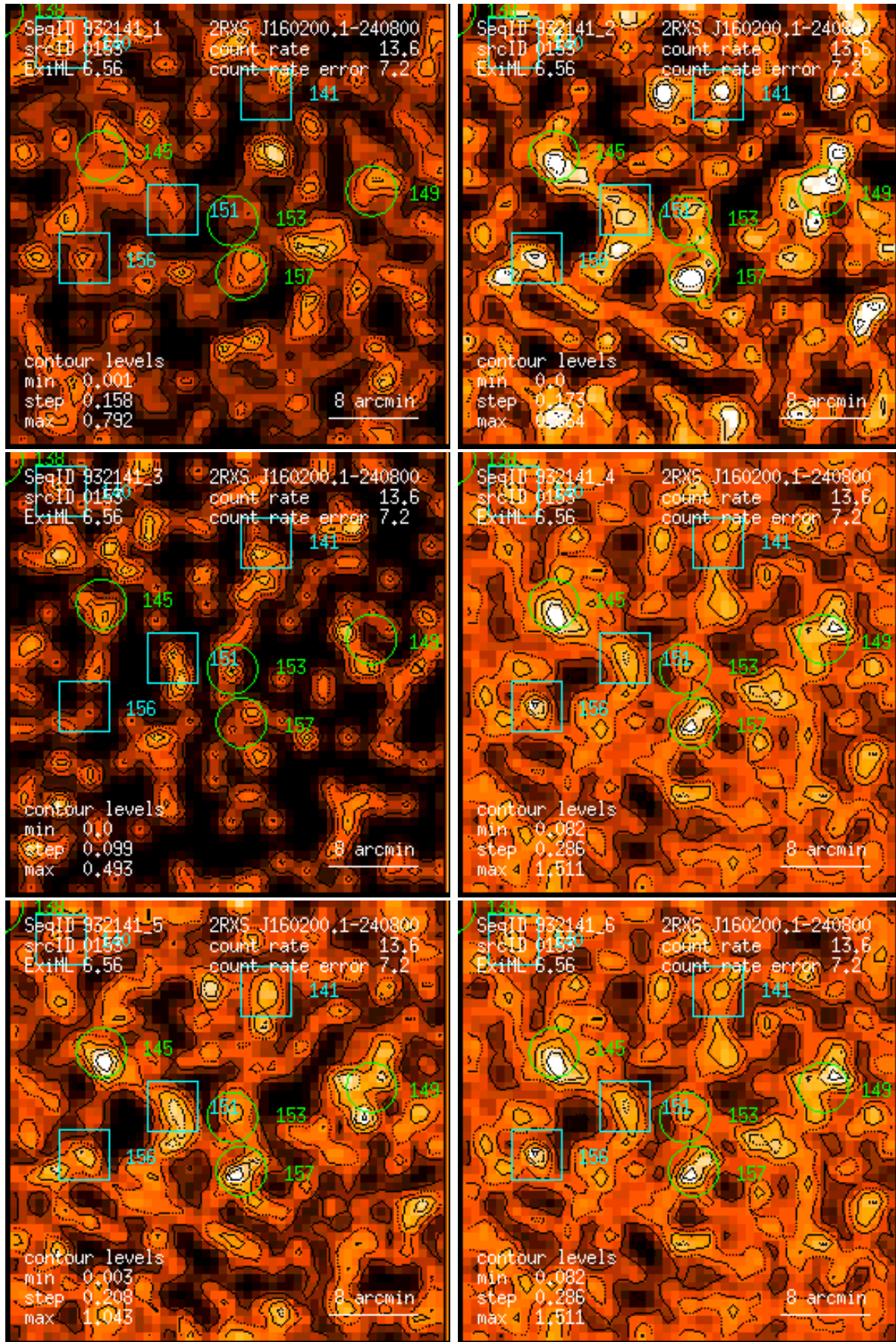
Figure 153: RASS 932141: detection 0153: band rate images, Gaussian filter: (1) PSPC channels 11 – 41, (2) 52 – 90, (3) 91 – 201, (4) 11 – 235, (5) 52 – 201, (6) 11 – 201. Broad band rates in counts/ks. Band rate contour levels in counts/ks/arcmin 2 .
