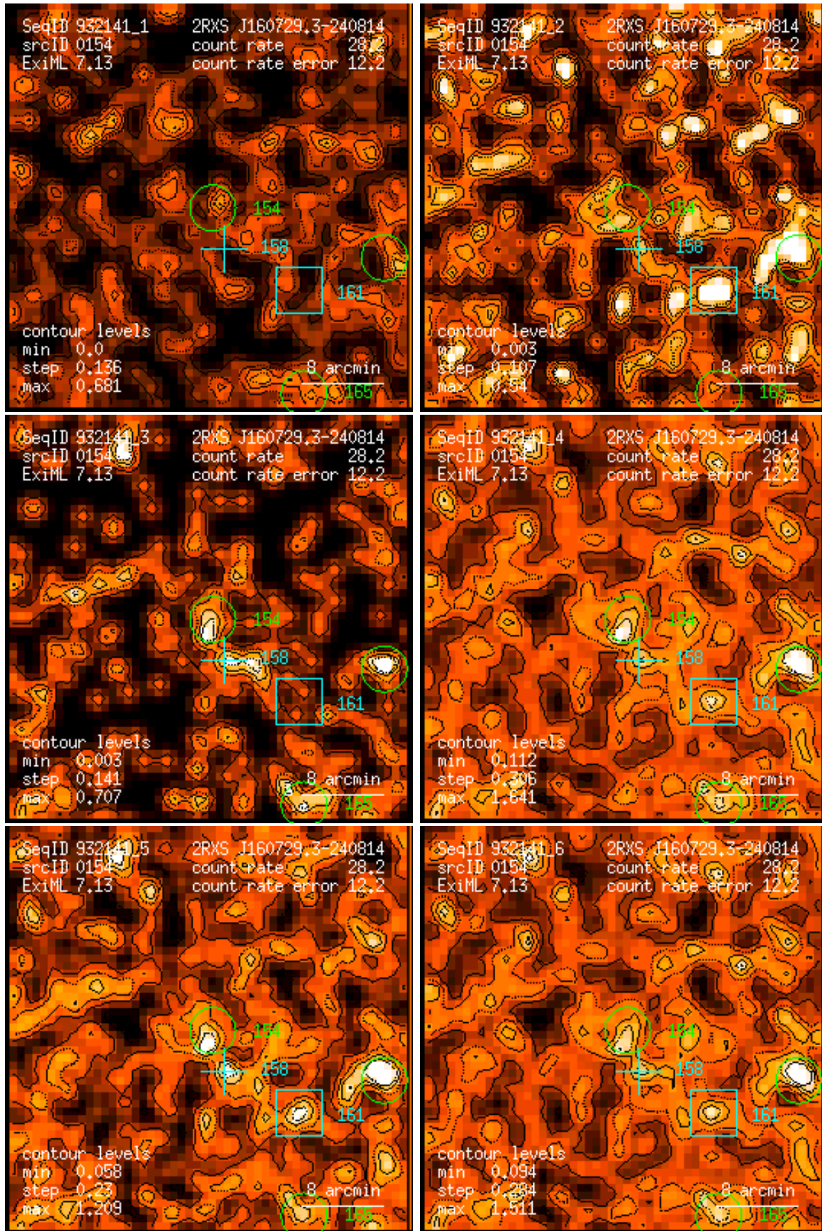
Figure 154: RASS 932141: detection 0154: band rate images, Gaussian filter: (1) PSPC channels 11 – 41, (2) 52 – 90, (3) 91 – 201, (4) 11 – 235, (5) 52 – 201, (6) 11 – 201. Broad band rates in counts/ks. Band rate contour levels in counts/ks/arcmin 2 .
