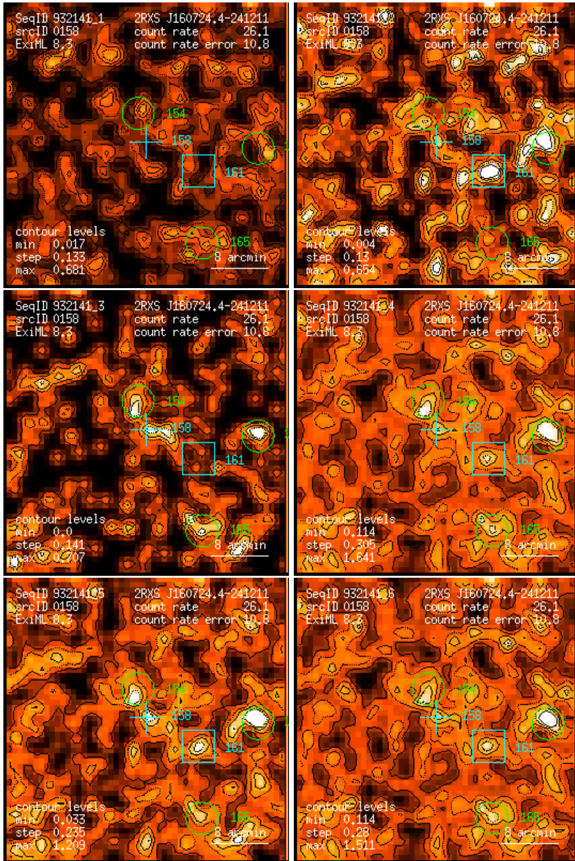
Figure 158: RASS 932141: detection 0158: band rate images, Gaussian filter: (1) PSPC channels 11 – 41, (2) 52 – 90, (3) 91 – 201, (4) 11 – 235, (5) 52 – 201, (6) 11 – 201. Broad band rates in counts/ks. Band rate contour levels in counts/ks/arcmin 2 .
