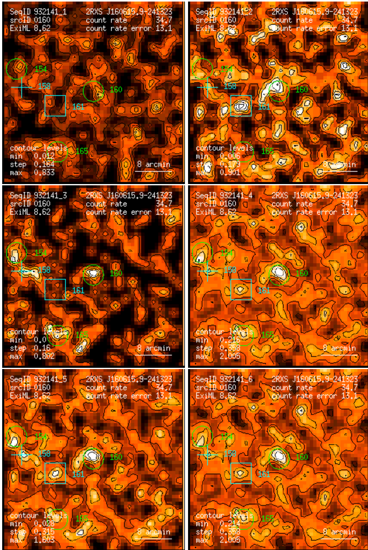
Figure 160: RASS 932141: detection 0160: band rate images, Gaussian filter: (1) PSPC channels 11 – 41, (2) 52 – 90, (3) 91 – 201, (4) 11 – 235, (5) 52 – 201, (6) 11 – 201. Broad band rates in counts/ks. Band rate contour levels in counts/ks/arcmin 2 .
