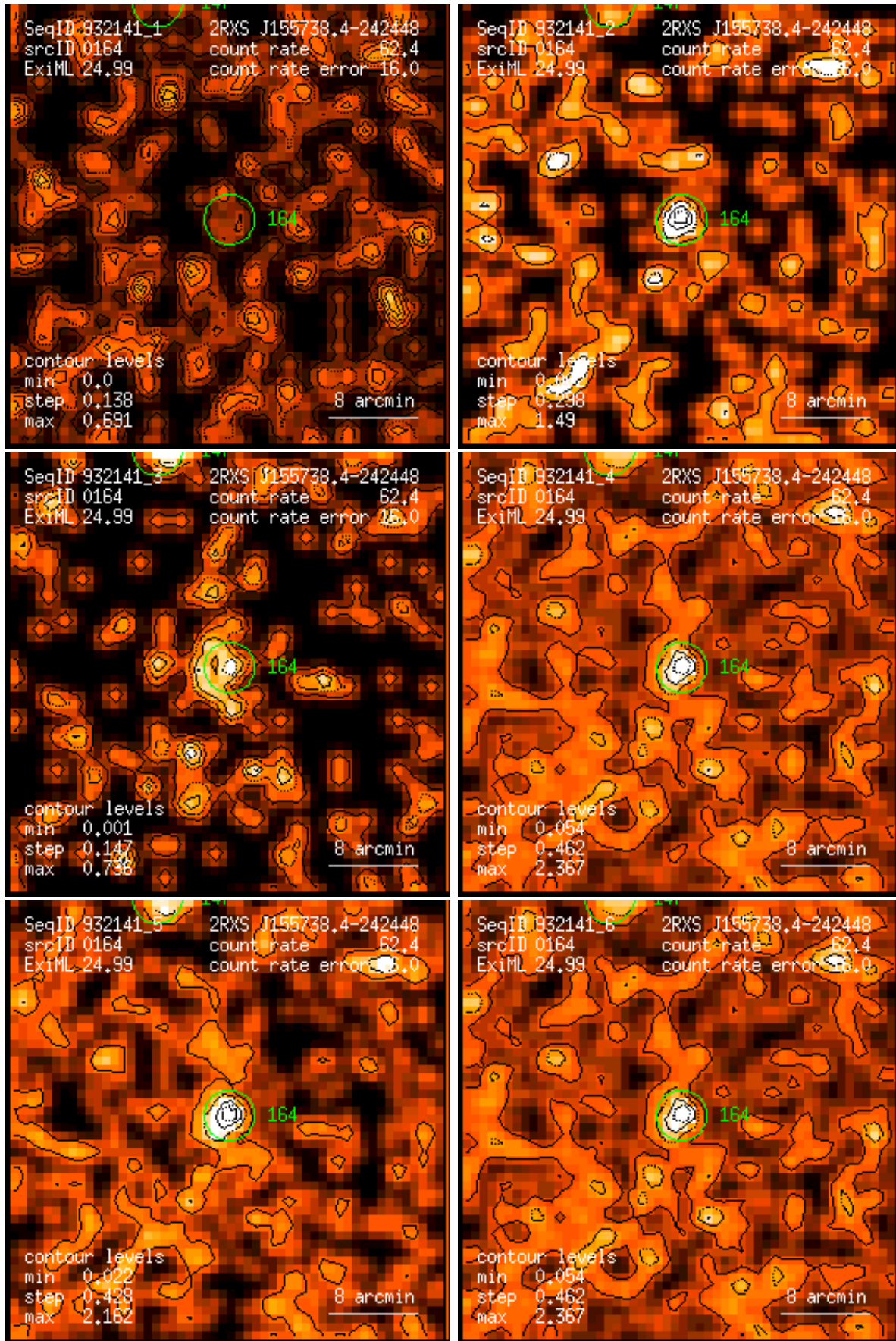
Figure 164: RASS 932141: detection 0164: band rate images, Gaussian filter: (1) PSPC channels 11 – 41, (2) 52 – 90, (3) 91 – 201, (4) 11 – 235, (5) 52 – 201, (6) 11 – 201. Broad band rates in counts/ks. Band rate contour levels in counts/ks/arcmin 2 .
