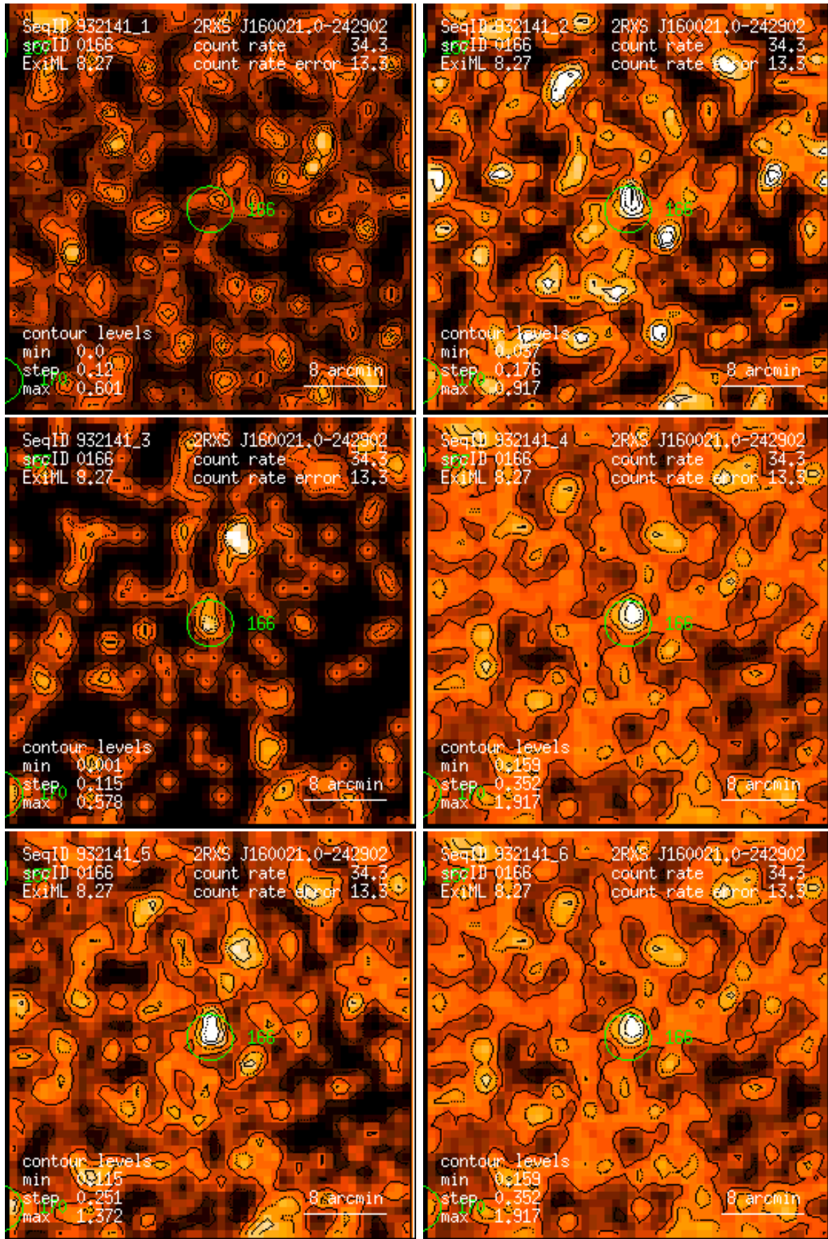
Figure 166: RASS 932141: detection 0166: band rate images, Gaussian filter: (1) PSPC channels 11 – 41, (2) 52 – 90, (3) 91 – 201, (4) 11 – 235, (5) 52 – 201, (6) 11 – 201. Broad band rates in counts/ks. Band rate contour levels in counts/ks/arcmin 2 .
