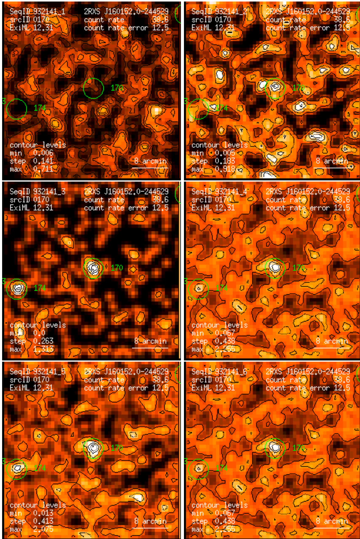
Figure 170: RASS 932141: detection 0170: band rate images, Gaussian filter: (1) PSPC channels 11 – 41, (2) 52 – 90, (3) 91 – 201, (4) 11 – 235, (5) 52 – 201, (6) 11 – 201. Broad band rates in counts/ks. Band rate contour levels in counts/ks/arcmin 2 .
