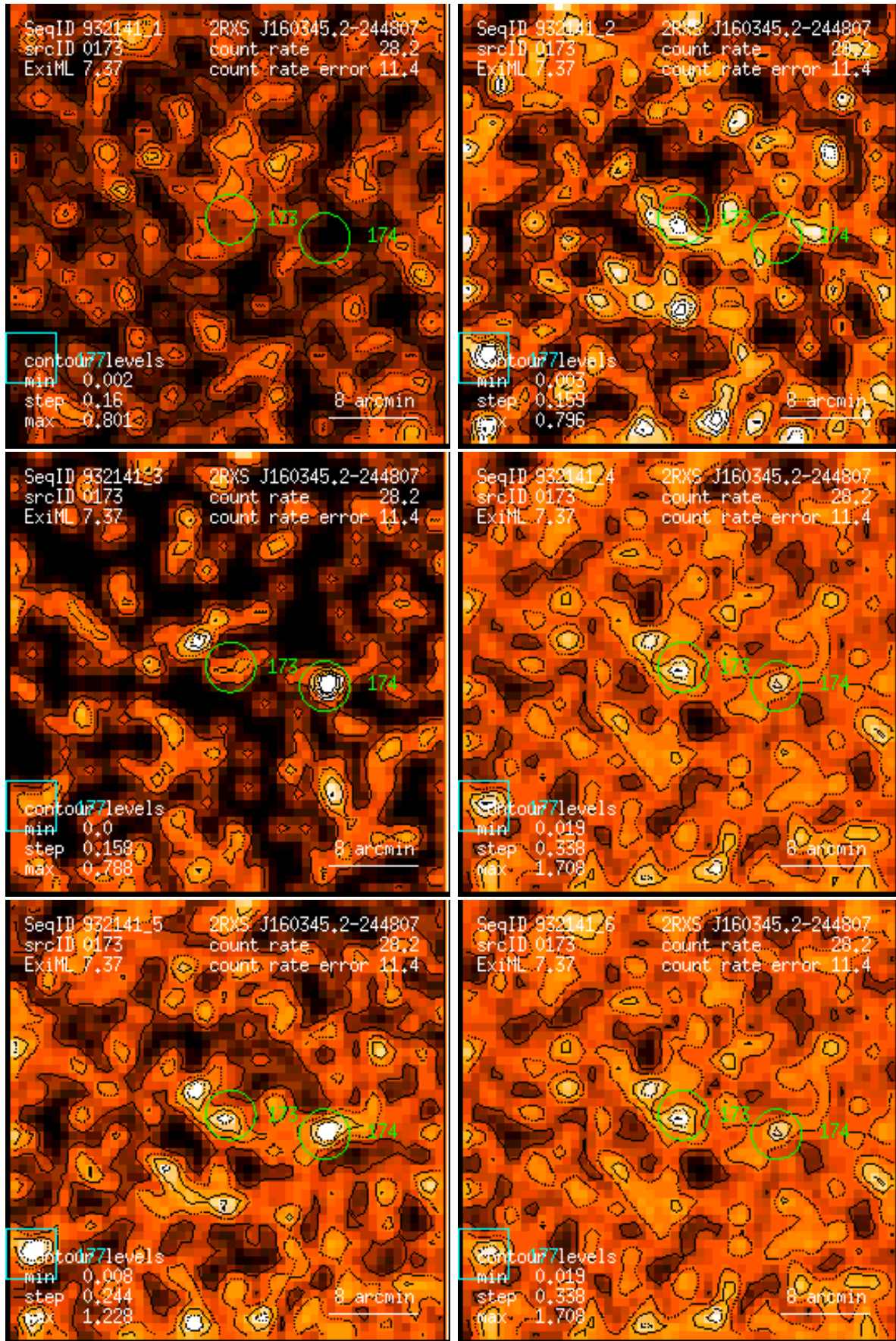
Figure 173: RASS 932141: detection 0173: band rate images, Gaussian filter: (1) PSPC channels 11 – 41, (2) 52 – 90, (3) 91 – 201, (4) 11 – 235, (5) 52 – 201, (6) 11 – 201. Broad band rates in counts/ks. Band rate contour levels in counts/ks/arcmin 2 .
