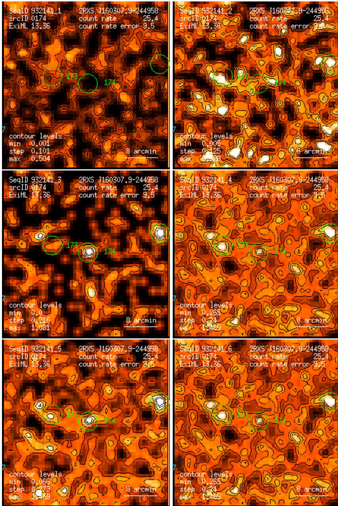
Figure 174: RASS 932141: detection 0174: band rate images, Gaussian filter: (1) PSPC channels 11 – 41, (2) 52 – 90, (3) 91 – 201, (4) 11 – 235, (5) 52 – 201, (6) 11 – 201. Broad band rates in counts/ks. Band rate contour levels in counts/ks/arcmin 2 .
