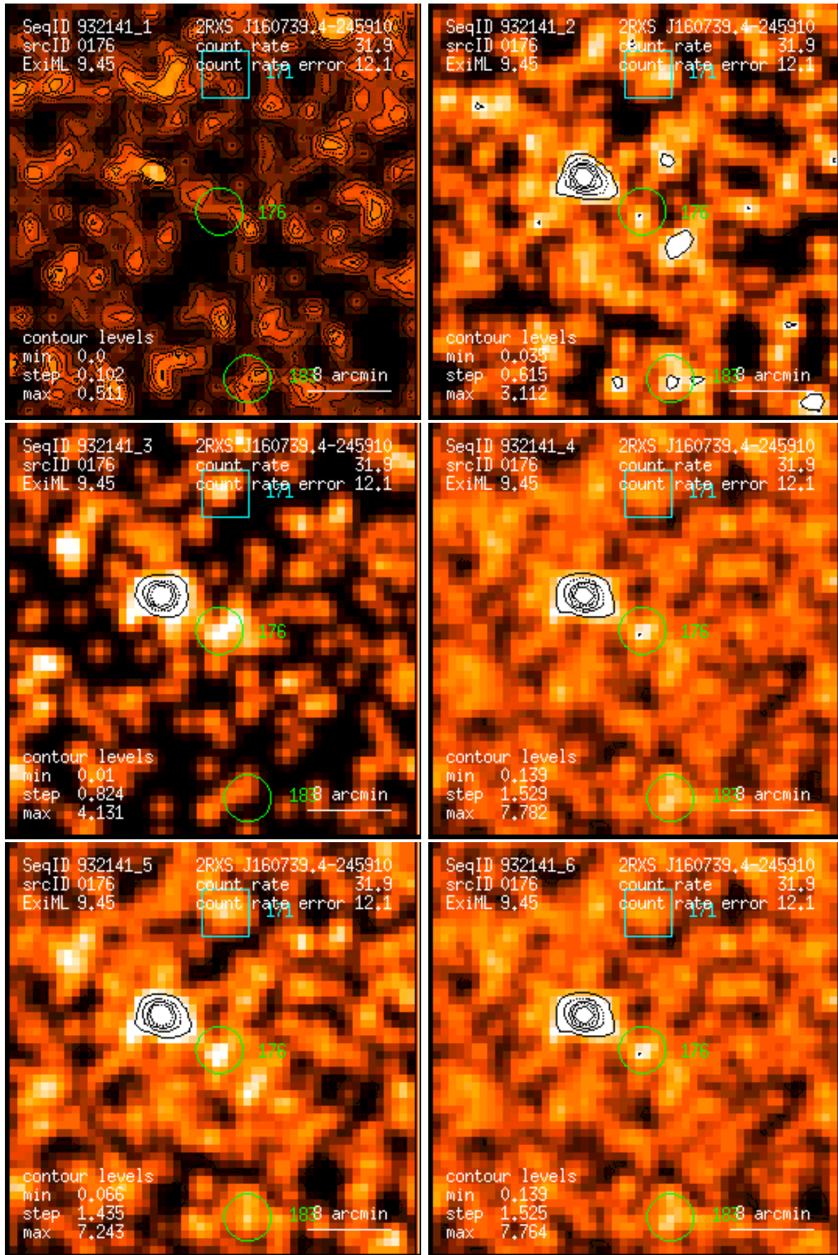
Figure 176: RASS 932141: detection 0176: band rate images, Gaussian filter: (1) PSPC channels 11 – 41, (2) 52 – 90, (3) 91 – 201, (4) 11 – 235, (5) 52 – 201, (6) 11 – 201. Broad band rates in counts/ks. Band rate contour levels in counts/ks/arcmin 2 .
