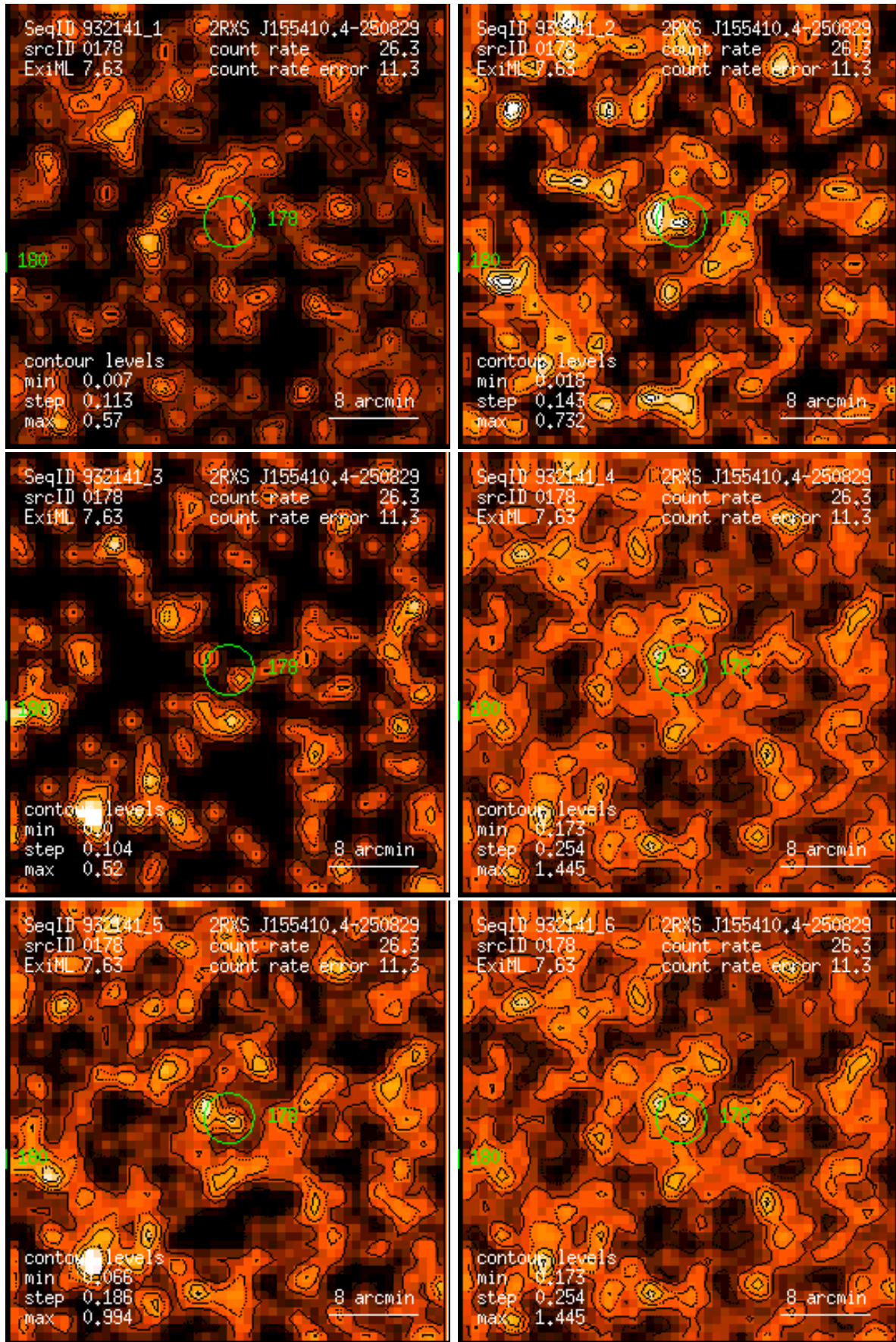
Figure 178: RASS 932141: detection 0178: band rate images, Gaussian filter: (1) PSPC channels 11 – 41, (2) 52 – 90, (3) 91 – 201, (4) 11 – 235, (5) 52 – 201, (6) 11 – 201. Broad band rates in counts/ks. Band rate contour levels in counts/ks/arcmin 2 .
