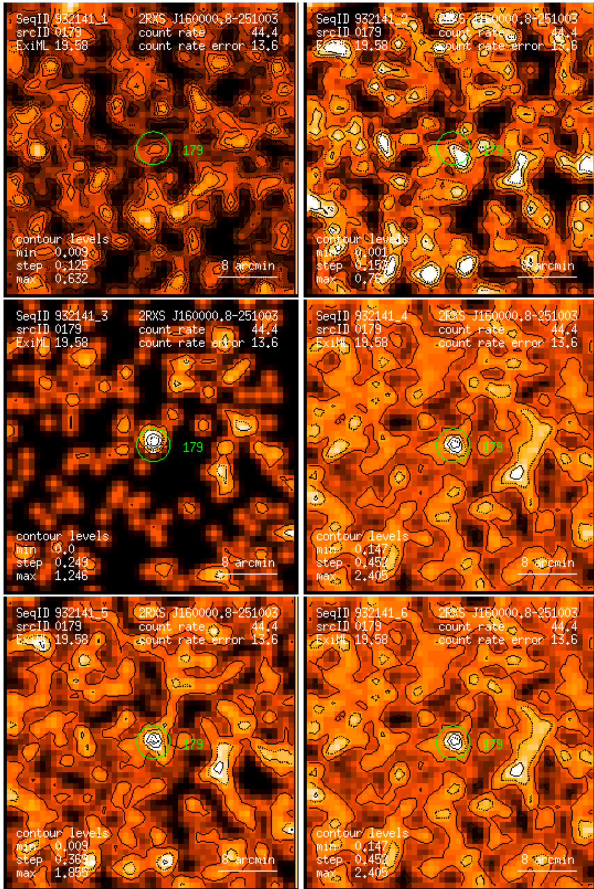
Figure 179: RASS 932141: detection 0179: band rate images, Gaussian filter: (1) PSPC channels 11 – 41, (2) 52 – 90, (3) 91 – 201, (4) 11 – 235, (5) 52 – 201, (6) 11 – 201. Broad band rates in counts/ks. Band rate contour levels in counts/ks/arcmin 2 .
