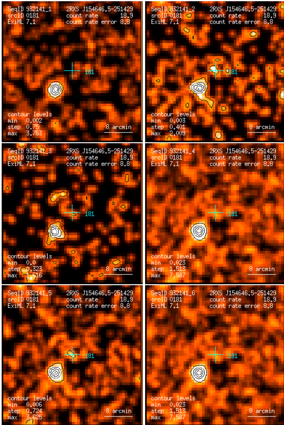
Figure 181: RASS 932141: detection 0181: band rate images, Gaussian filter: (1) PSPC channels 11 – 41, (2) 52 – 90, (3) 91 – 201, (4) 11 – 235, (5) 52 – 201, (6) 11 – 201. Broad band rates in counts/ks. Band rate contour levels in counts/ks/arcmin 2 .
