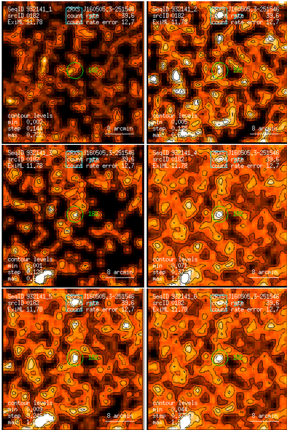
Figure 182: RASS 932141: detection 0182: band rate images, Gaussian filter: (1) PSPC channels 11 – 41, (2) 52 – 90, (3) 91 – 201, (4) 11 – 235, (5) 52 – 201, (6) 11 – 201. Broad band rates in counts/ks. Band rate contour levels in counts/ks/arcmin 2 .
