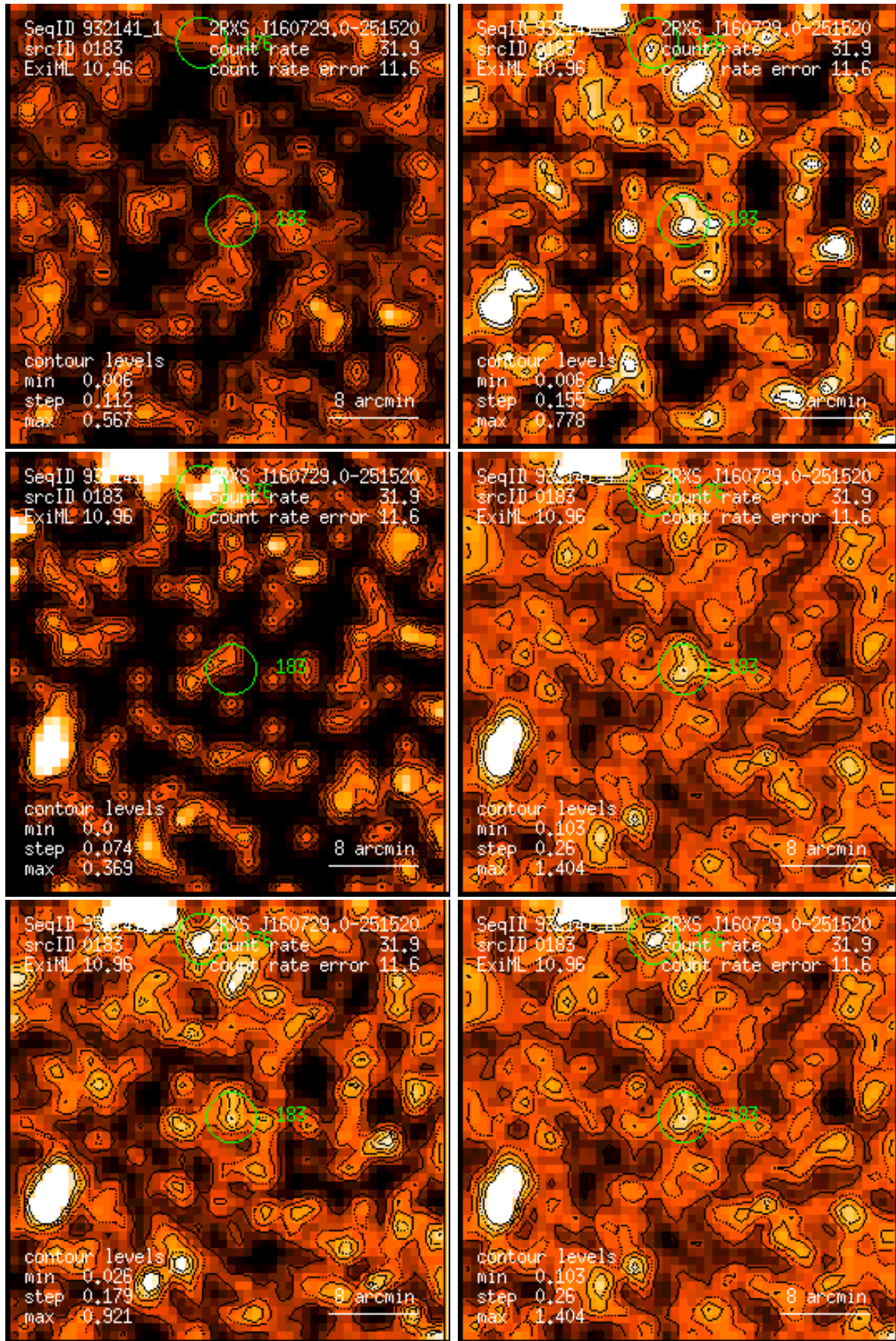
Figure 183: RASS 932141: detection 0183: band rate images, Gaussian filter: (1) PSPC channels 11 – 41, (2) 52 – 90, (3) 91 – 201, (4) 11 – 235, (5) 52 – 201, (6) 11 – 201. Broad band rates in counts/ks. Band rate contour levels in counts/ks/arcmin 2 .
