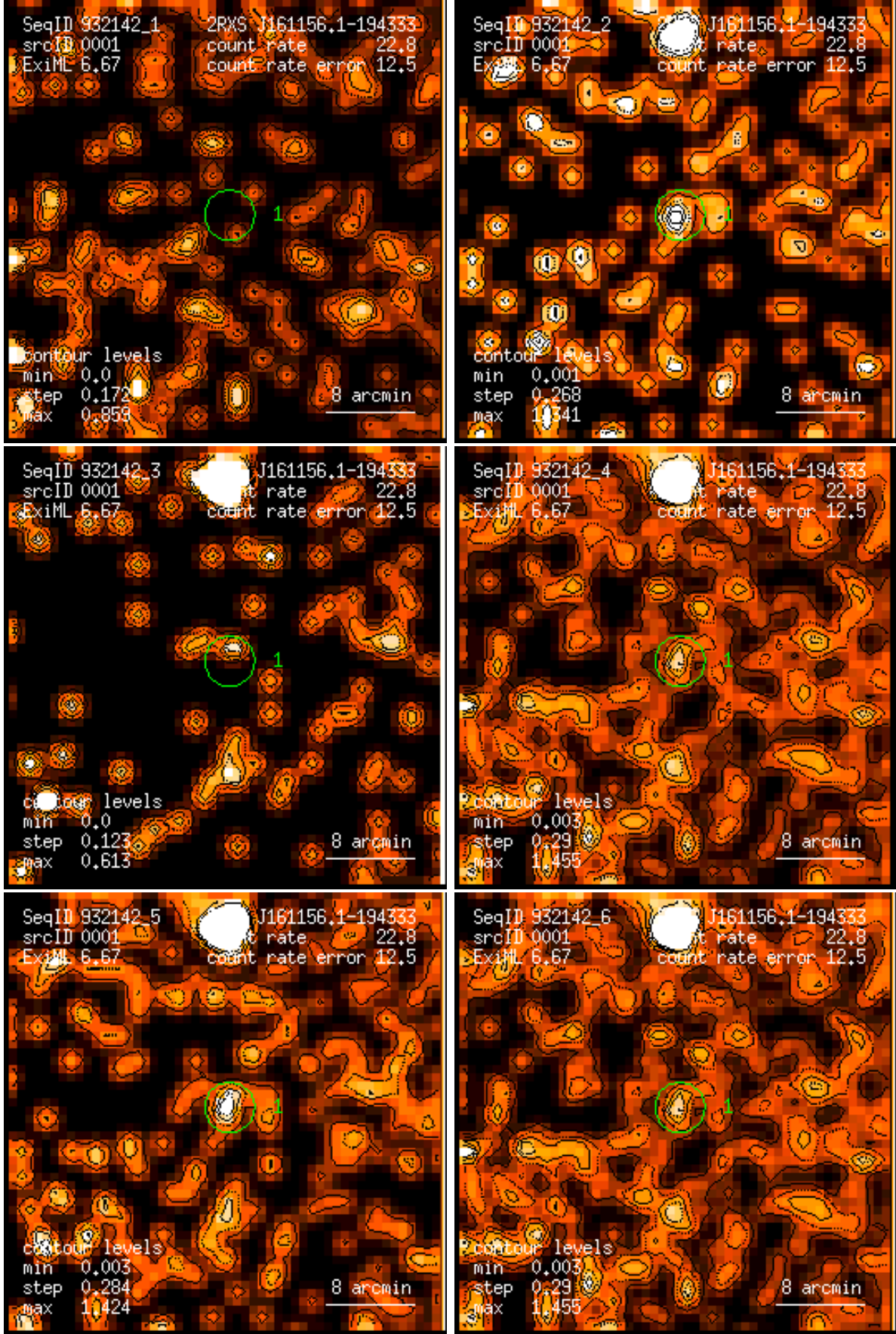
Figure 1: RASS 932142: detection 0001: band rate images, Gaussian filter: (1) PSPC channels 11 – 41, (2) 52 – 90, (3) 91 – 201, (4) 11 – 235, (5) 52 – 201, (6) 11 – 201. Broad band rates in counts/ks. Band rate contour levels in counts/ks/arcmin 2 .
