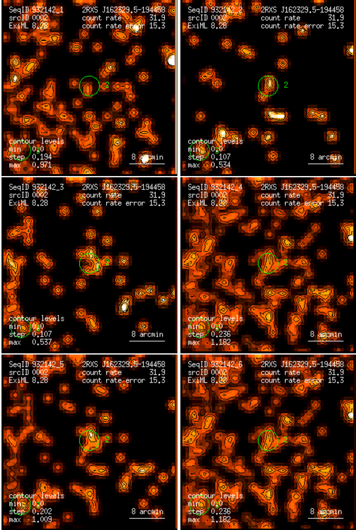
Figure 2: RASS 932142: detection 0002: band rate images, Gaussian filter: (1) PSPC channels 11 – 41, (2) 52 – 90, (3) 91 – 201, (4) 11 – 235, (5) 52 – 201, (6) 11 – 201. Broad band rates in counts/ks. Band rate contour levels in counts/ks/arcmin 2 .
