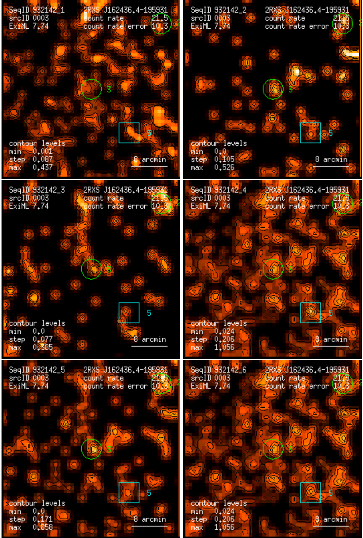
Figure 3: RASS 932142: detection 0003: band rate images, Gaussian filter: (1) PSPC channels 11 – 41, (2) 52 – 90, (3) 91 – 201, (4) 11 – 235, (5) 52 – 201, (6) 11 – 201. Broad band rates in counts/ks. Band rate contour levels in counts/ks/arcmin 2 .
