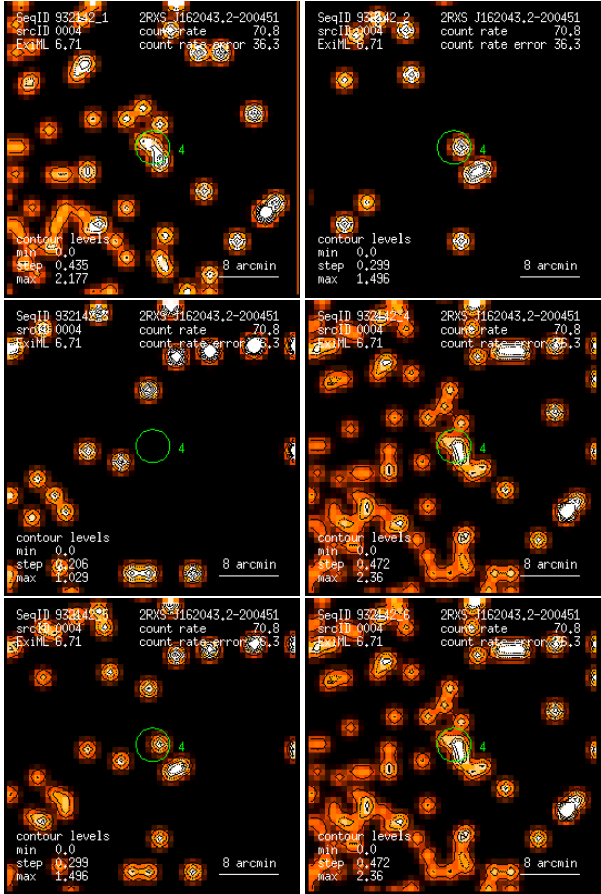
Figure 4: RASS 932142: detection 0004: band rate images, Gaussian filter: (1) PSPC channels 11 – 41, (2) 52 – 90, (3) 91 – 201, (4) 11 – 235, (5) 52 – 201, (6) 11 – 201. Broad band rates in counts/ks. Band rate contour levels in counts/ks/arcmin 2 .
