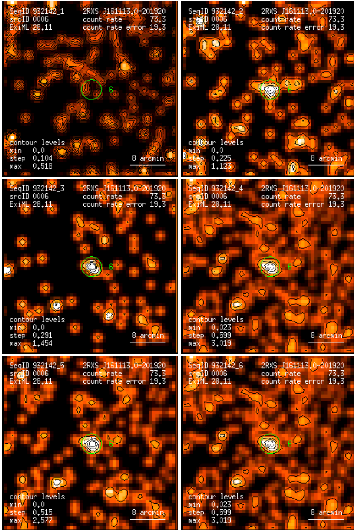
Figure 6: RASS 932142: detection 0006: band rate images, Gaussian filter: (1) PSPC channels 11 – 41, (2) 52 – 90, (3) 91 – 201, (4) 11 – 235, (5) 52 – 201, (6) 11 – 201. Broad band rates in counts/ks. Band rate contour levels in counts/ks/arcmin 2 .
