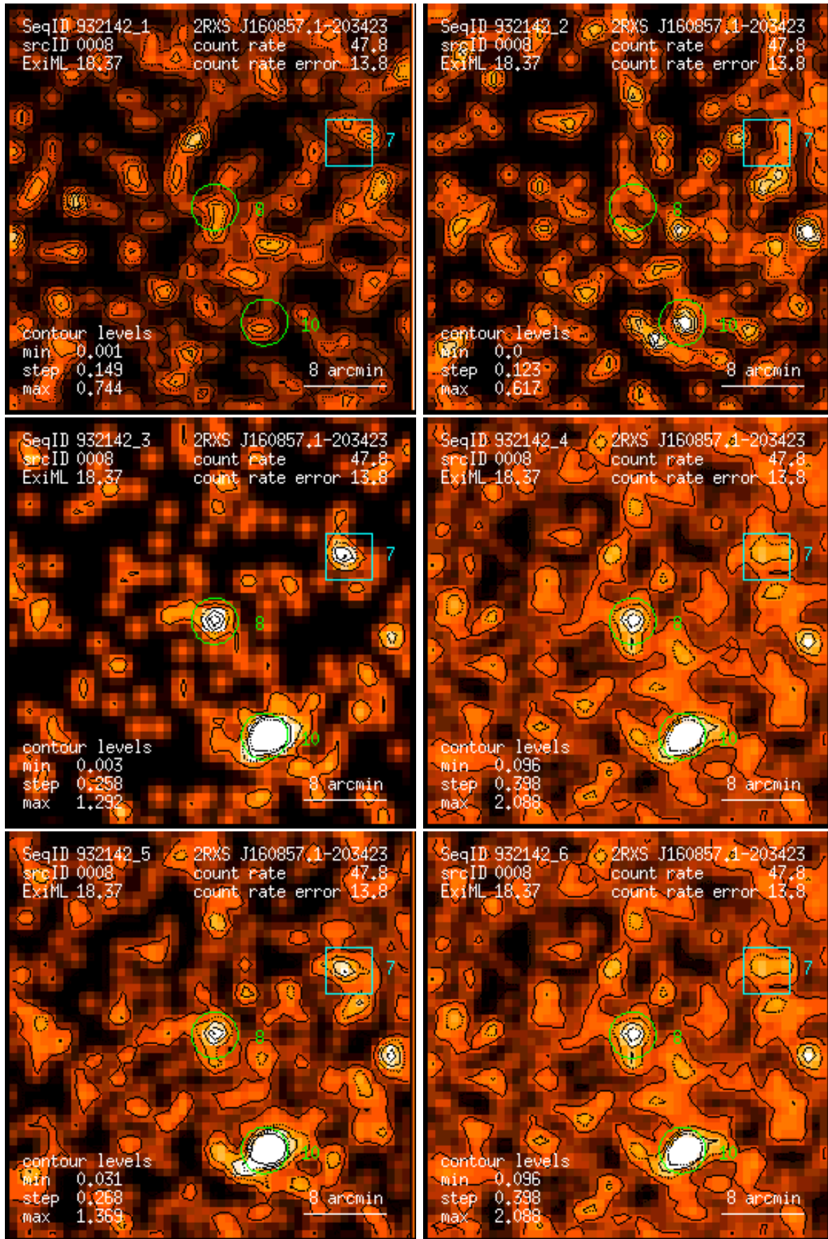
Figure 8: RASS 932142: detection 0008: band rate images, Gaussian filter: (1) PSPC channels 11 – 41, (2) 52 – 90, (3) 91 – 201, (4) 11 – 235, (5) 52 – 201, (6) 11 – 201. Broad band rates in counts/ks. Band rate contour levels in counts/ks/arcmin 2 .
