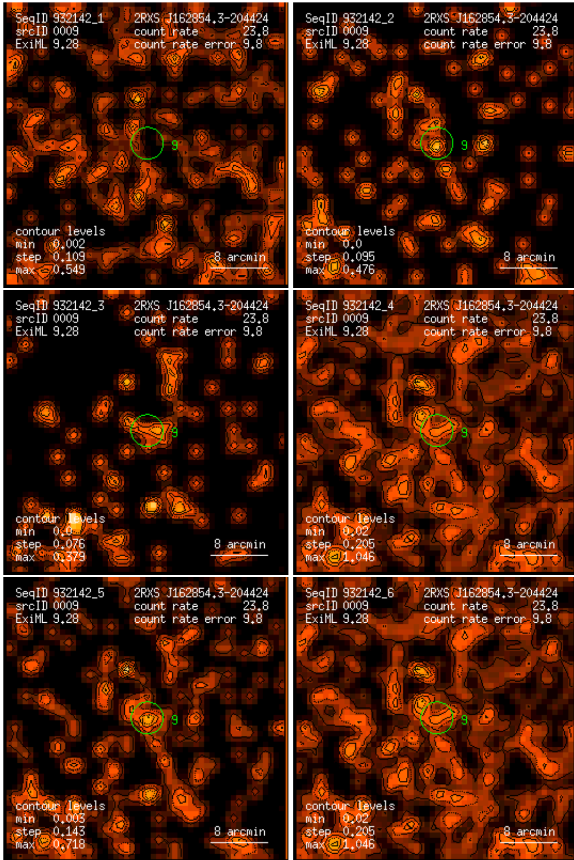
Figure 9: RASS 932142: detection 0009: band rate images, Gaussian filter: (1) PSPC channels 11 – 41, (2) 52 – 90, (3) 91 – 201, (4) 11 – 235, (5) 52 – 201, (6) 11 – 201. Broad band rates in counts/ks. Band rate contour levels in counts/ks/arcmin 2 .
