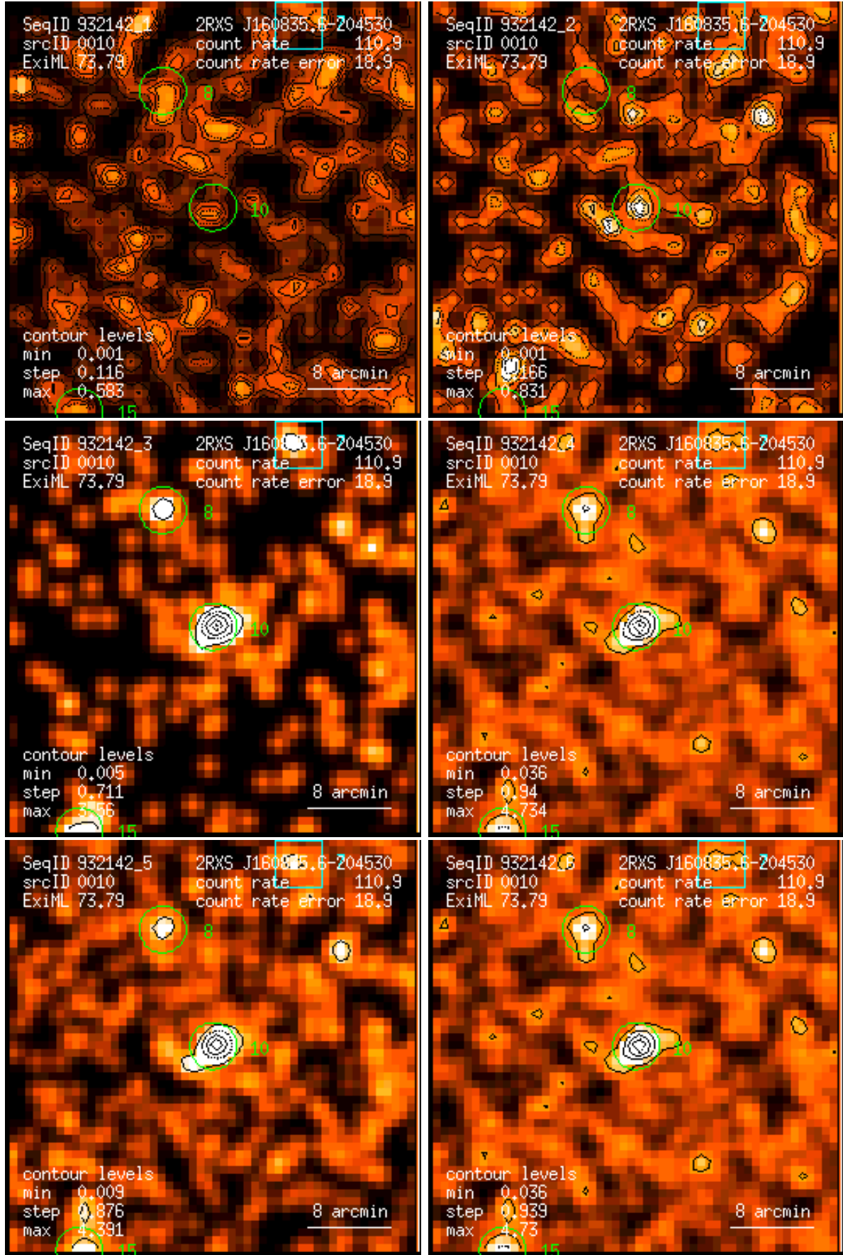
Figure 10: RASS 932142: detection 0010: band rate images, Gaussian filter: (1) PSPC channels 11 – 41, (2) 52 – 90, (3) 91 – 201, (4) 11 – 235, (5) 52 – 201, (6) 11 – 201. Broad band rates in counts/ks. Band rate contour levels in counts/ks/arcmin 2 .
