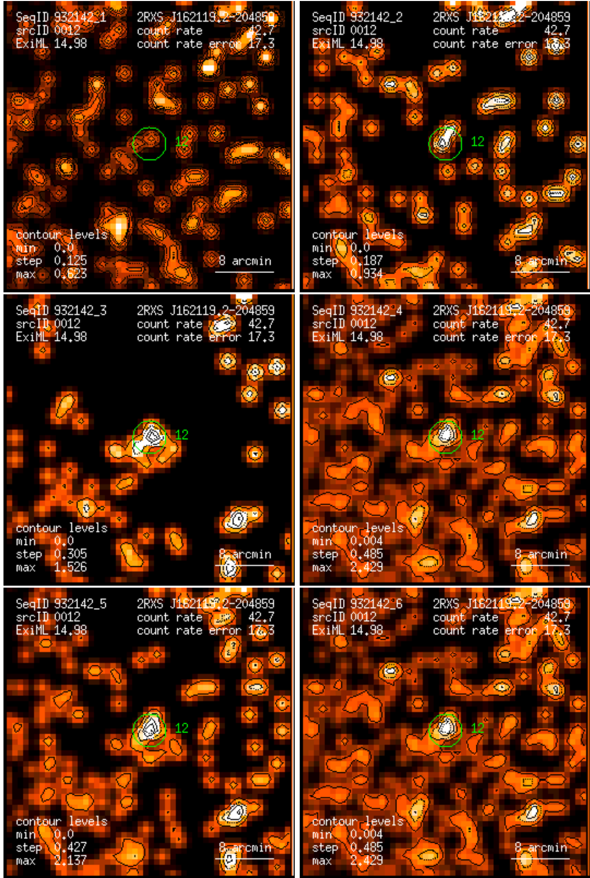
Figure 12: RASS 932142: detection 0012: band rate images, Gaussian filter: (1) PSPC channels 11 – 41, (2) 52 – 90, (3) 91 – 201, (4) 11 – 235, (5) 52 – 201, (6) 11 – 201. Broad band rates in counts/ks. Band rate contour levels in counts/ks/arcmin 2 .
