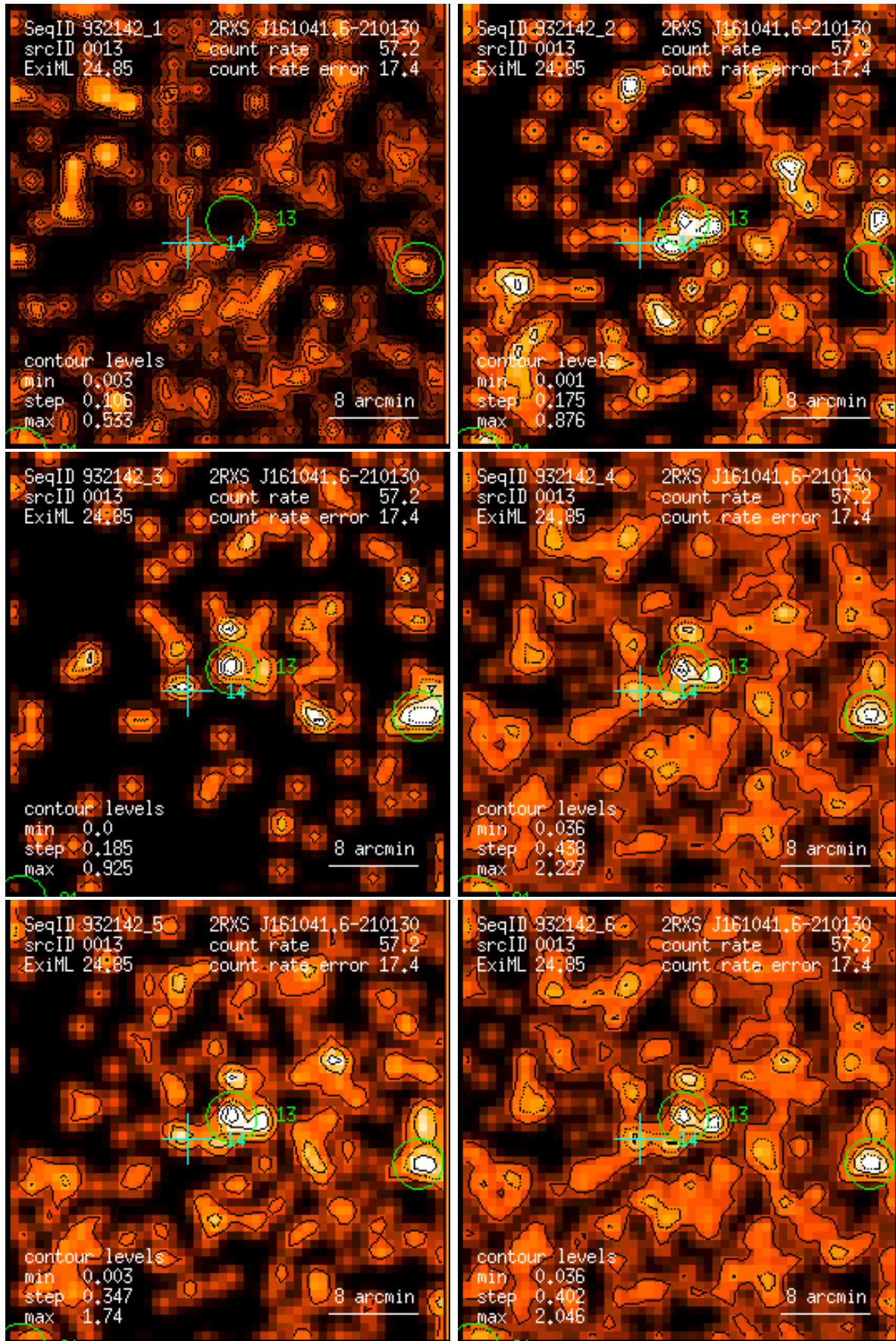
Figure 13: RASS 932142: detection 0013: band rate images, Gaussian filter: (1) PSPC channels 11 – 41, (2) 52 – 90, (3) 91 – 201, (4) 11 – 235, (5) 52 – 201, (6) 11 – 201. Broad band rates in counts/ks. Band rate contour levels in counts/ks/arcmin 2 .
