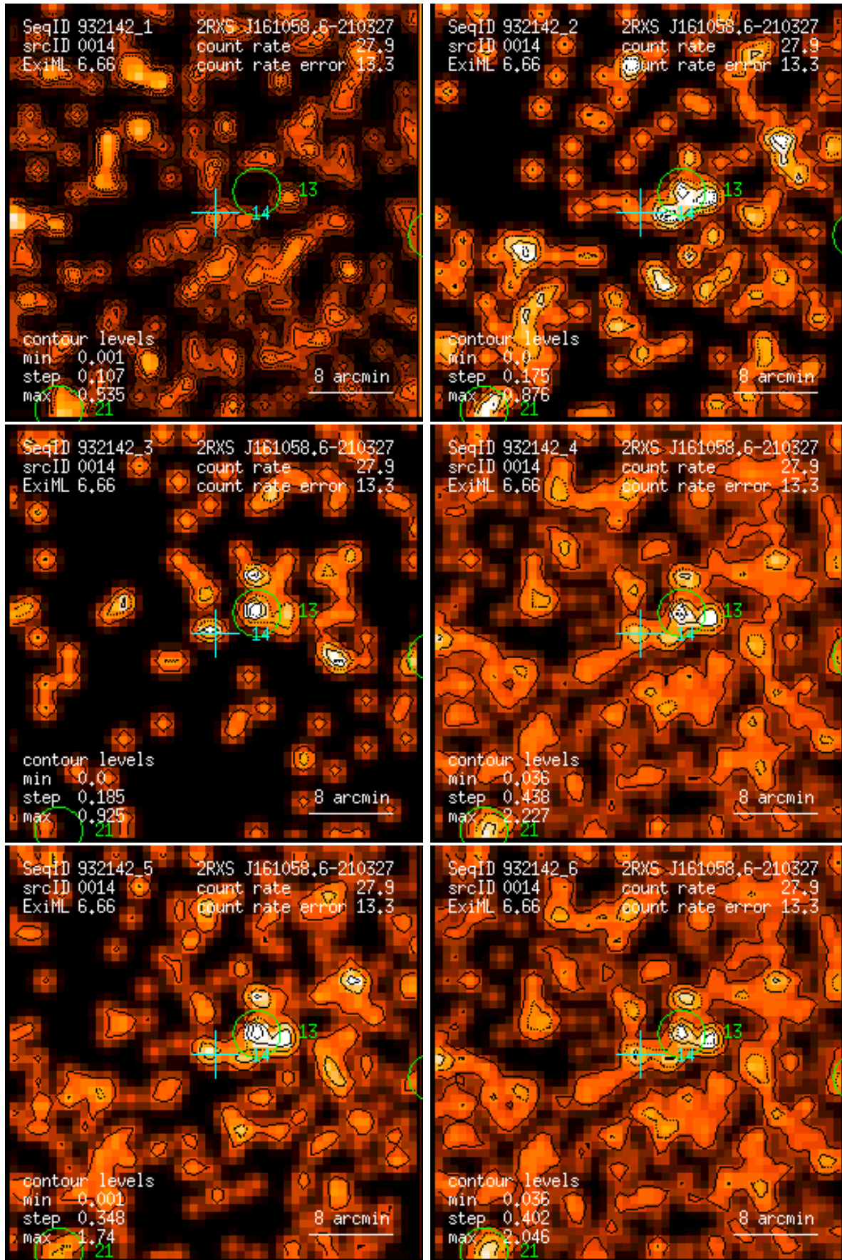
Figure 14: RASS 932142: detection 0014: band rate images, Gaussian filter: (1) PSPC channels 11 – 41, (2) 52 – 90, (3) 91 – 201, (4) 11 – 235, (5) 52 – 201, (6) 11 – 201. Broad band rates in counts/ks. Band rate contour levels in counts/ks/arcmin 2 .
