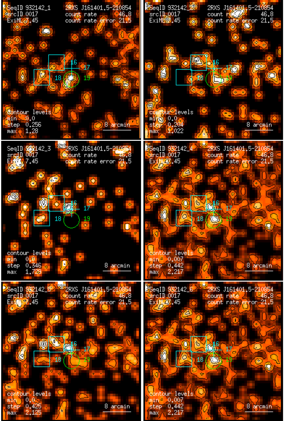
Figure 17: RASS 932142: detection 0017: band rate images, Gaussian filter: (1) PSPC channels 11 – 41, (2) 52 – 90, (3) 91 – 201, (4) 11 – 235, (5) 52 – 201, (6) 11 – 201. Broad band rates in counts/ks. Band rate contour levels in counts/ks/arcmin 2 .
