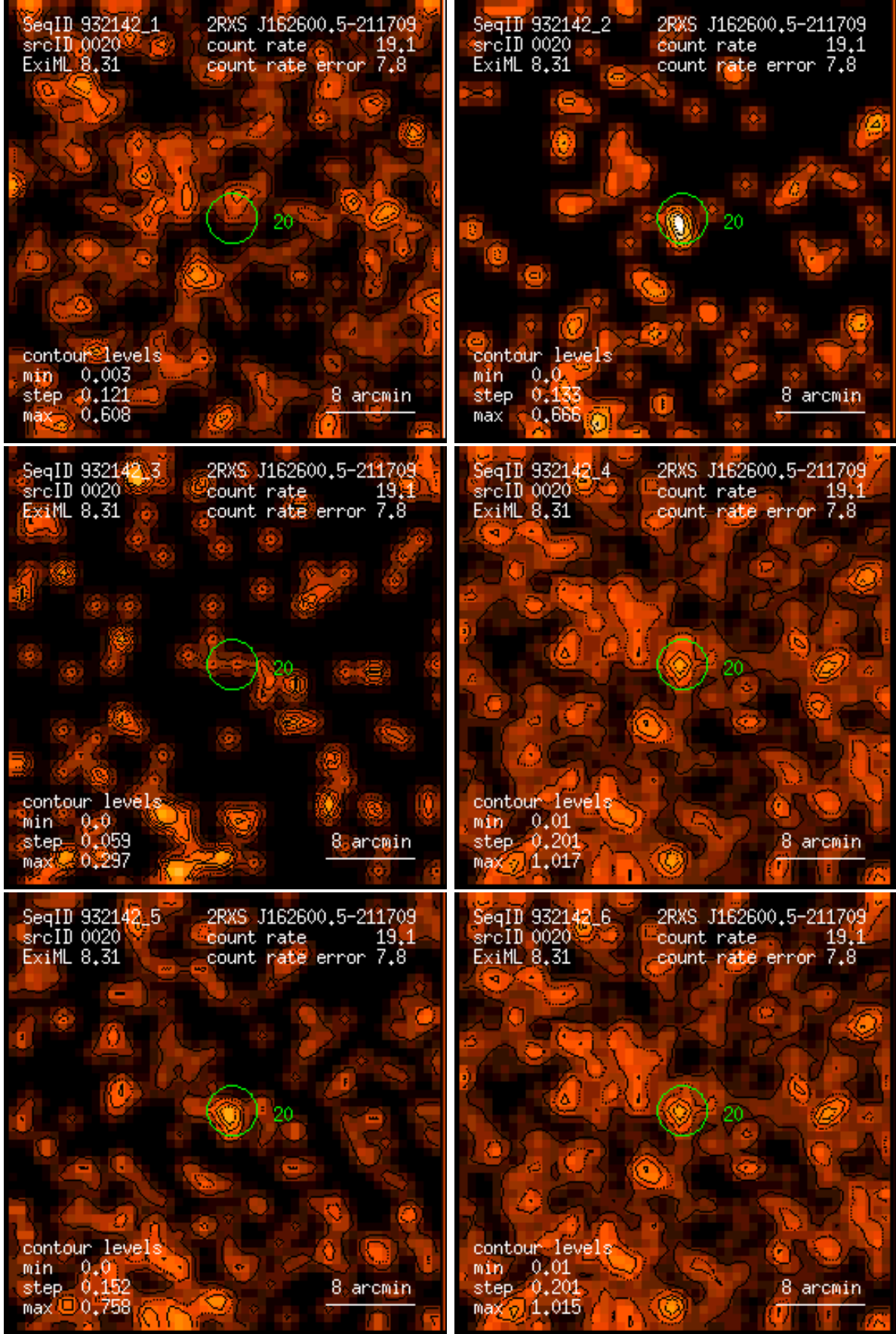
Figure 20: RASS 932142: detection 0020: band rate images, Gaussian filter: (1) PSPC channels 11 – 41, (2) 52 – 90, (3) 91 – 201, (4) 11 – 235, (5) 52 – 201, (6) 11 – 201. Broad band rates in counts/ks. Band rate contour levels in counts/ks/arcmin 2 .
