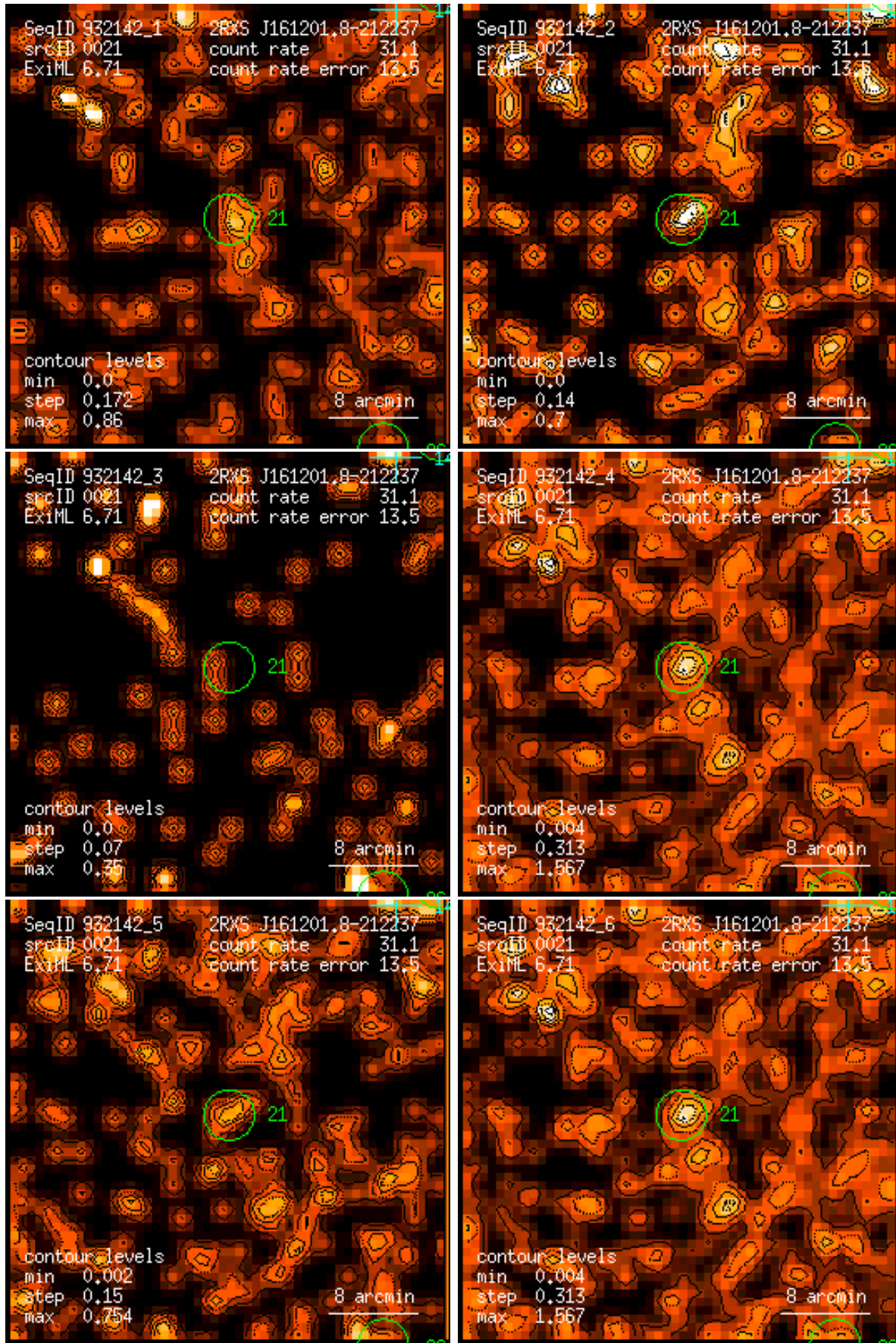
Figure 21: RASS 932142: detection 0021: band rate images, Gaussian filter: (1) PSPC channels 11 – 41, (2) 52 – 90, (3) 91 – 201, (4) 11 – 235, (5) 52 – 201, (6) 11 – 201. Broad band rates in counts/ks. Band rate contour levels in counts/ks/arcmin 2 .
