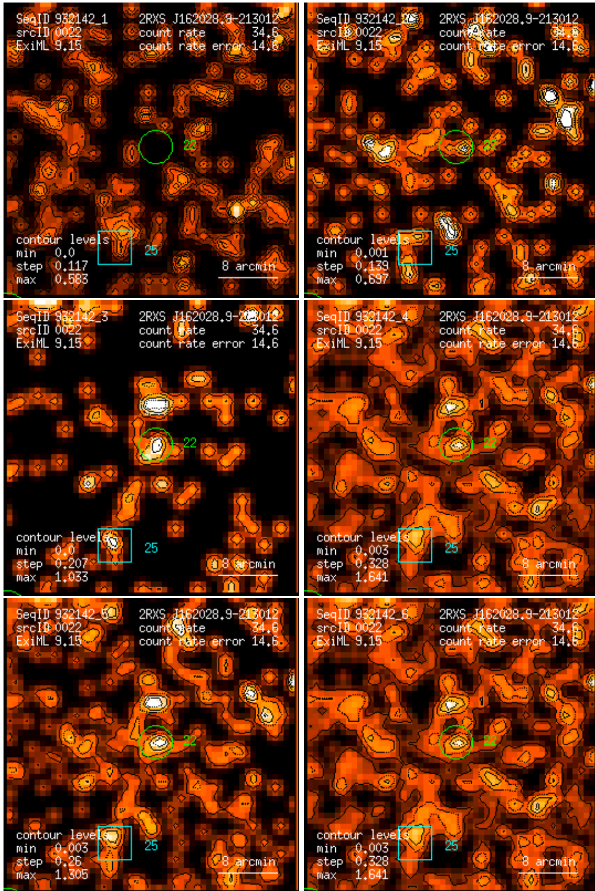
Figure 22: RASS 932142: detection 0022: band rate images, Gaussian filter: (1) PSPC channels 11 – 41, (2) 52 – 90, (3) 91 – 201, (4) 11 – 235, (5) 52 – 201, (6) 11 – 201. Broad band rates in counts/ks. Band rate contour levels in counts/ks/arcmin 2 .
