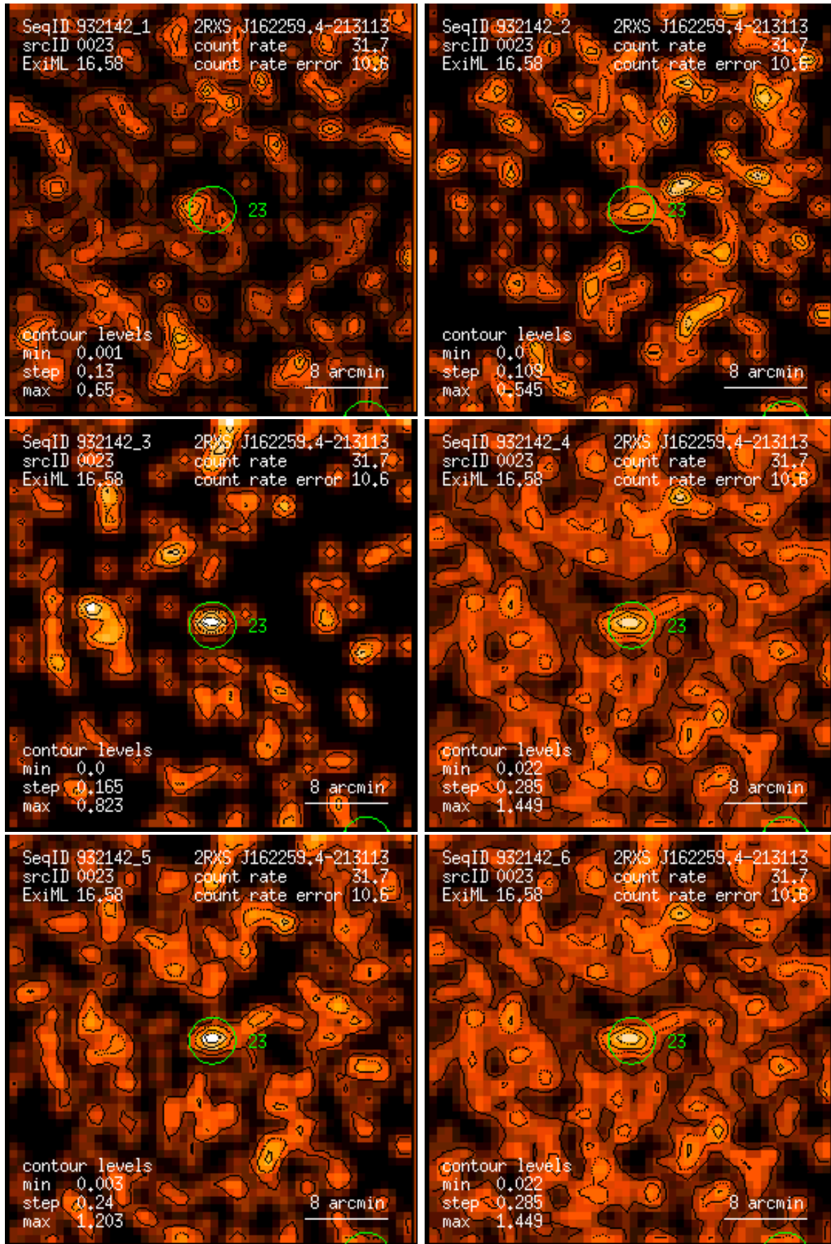
Figure 23: RASS 932142: detection 0023: band rate images, Gaussian filter: (1) PSPC channels 11 – 41, (2) 52 – 90, (3) 91 – 201, (4) 11 – 235, (5) 52 – 201, (6) 11 – 201. Broad band rates in counts/ks. Band rate contour levels in counts/ks/arcmin 2 .
