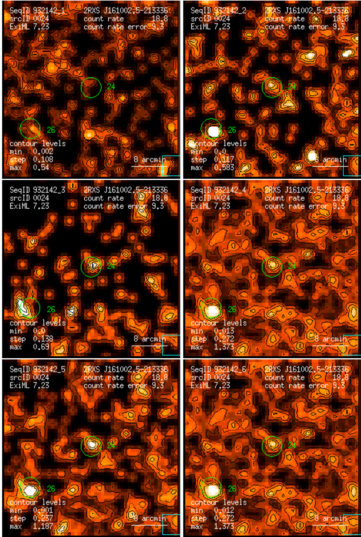
Figure 24: RASS 932142: detection 0024: band rate images, Gaussian filter: (1) PSPC channels 11 – 41, (2) 52 – 90, (3) 91 – 201, (4) 11 – 235, (5) 52 – 201, (6) 11 – 201. Broad band rates in counts/ks. Band rate contour levels in counts/ks/arcmin 2 .
